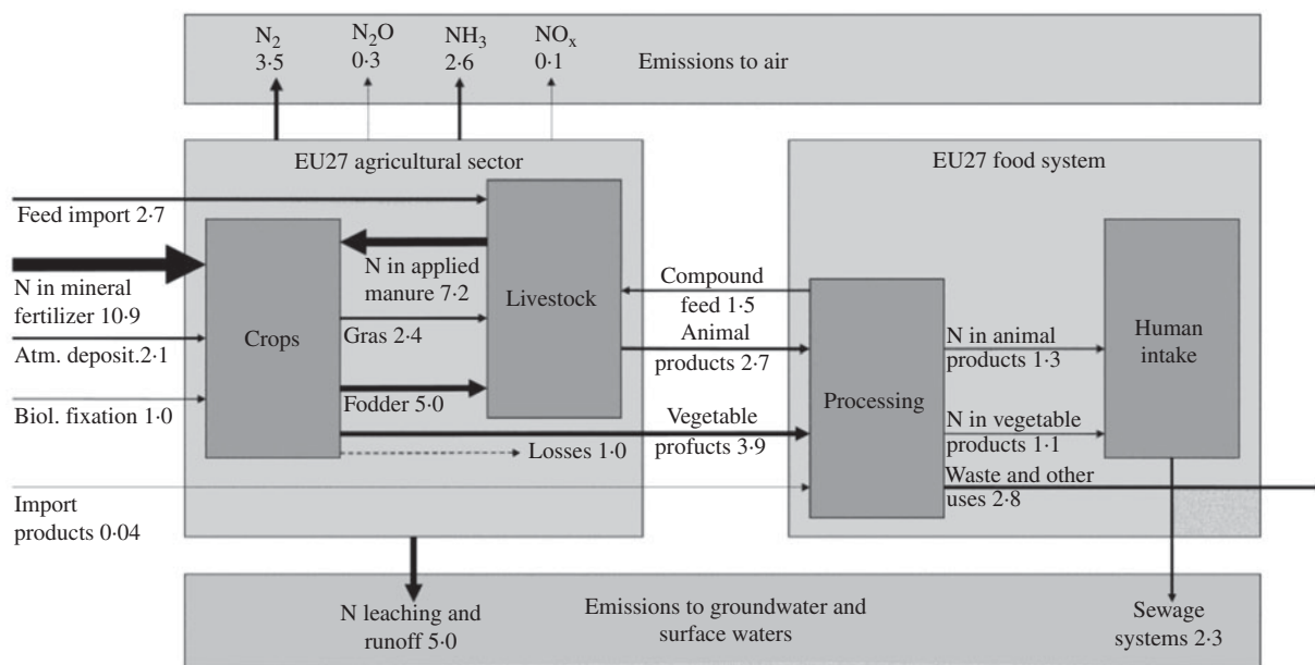
Fig. 1. Nitrogen flows (Mt N/year) in the agricultural sector of EU27. Reference year: 2004.
