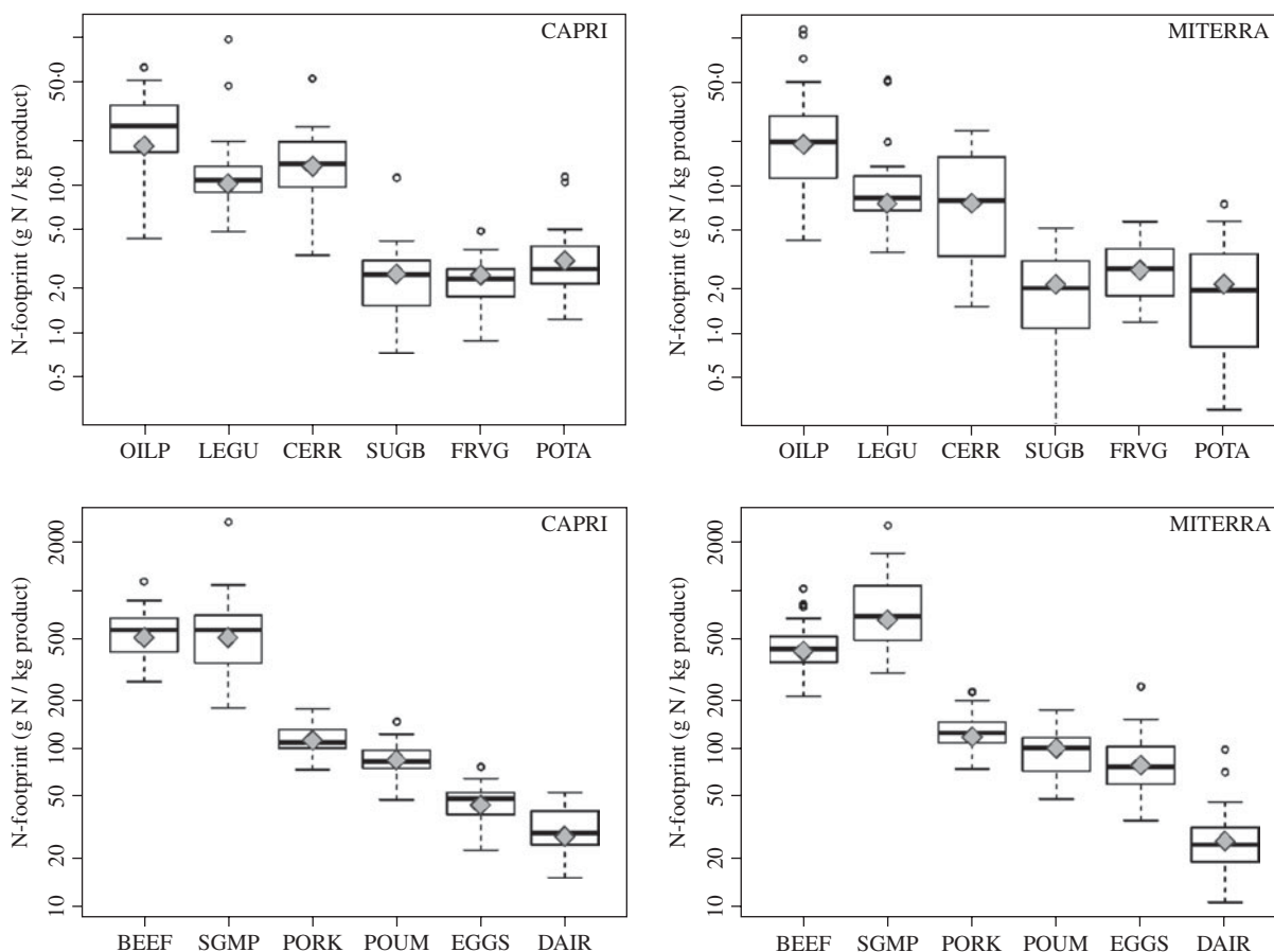
Fig. 2. Nitrogen footprint for the 12 main food commodity groups (g N/kg product). Left: CAPRI; right: MITERRA. The box-whisker diagram shows the median and lower and upper quartiles (boxes) and the minimum and maximum of the sample (whiskers) excluding outliers. Outliers (more than 1.5 times the quartiles) are shown as circles. The values for EU25, calculated as weighted average, are shown as diamonds. Note the logarithmic scale of the y-axis.
