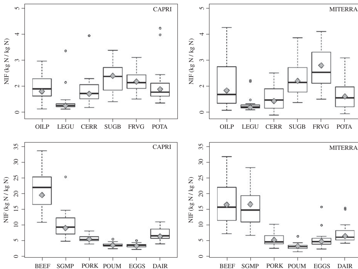
Fig. 4. Nitrogen investment factor for the 12 main food categories (kg N input/kg N in product). Left: CAPRI; right: MITERRA. The box-whisker diagram shows the median and lower and upper quartiles (boxes) and the minimum and maximum of the sample (whiskers) excluding outliers. Outliers (more than 1.5 times the quartiles) are shown as circles. The values for EU27, calculated as weighted average, are shown as diamonds.
