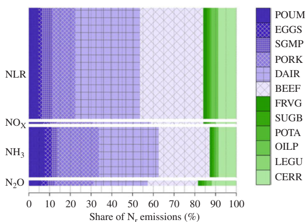
Fig. 3. Share of reactive nitrogen emissions for the 12 main food commodity groups as calculated with the CAPRI model (reference year 2004). The width of the bars is proportional to the emissions. Total emissions are N_2O : 0.29 Tg N/year; NH_3 : 2.8 Tg N/year; NO_x : 0.09 Tg N/year; N leaching and run-off (NLR): 6.3 Tg N/year; other nitrogen considered in the N footprint losses ( N_2 emissions, manure and animal wastes), but not shown: 5.3 Tg N/year. (colour version available online)
