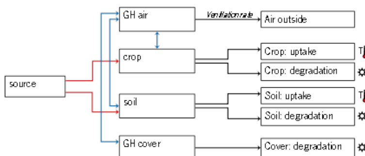
Figure 1. Schematic view of the VEGA model. Boxes marked with T represent temperature dependent processes; boxes marked with a small sun pictogram represent processes that are dependent on solar radiation.
