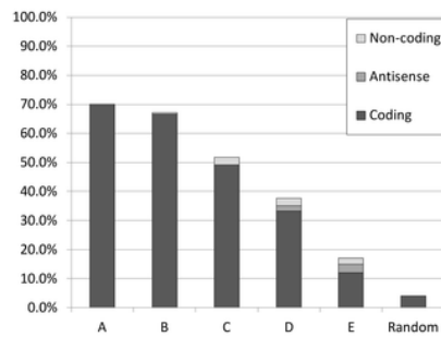
Figure 4. Frequency distribution of validated promoters.
