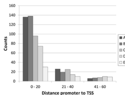
Figure 3. Distribution of distances between promoters and TSSs.
