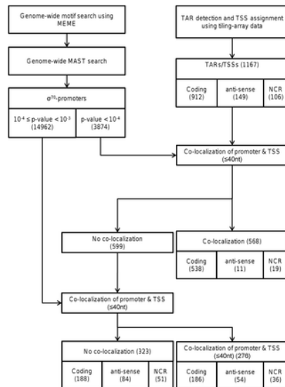
Figure 2. Flow chart of promoter validation.
