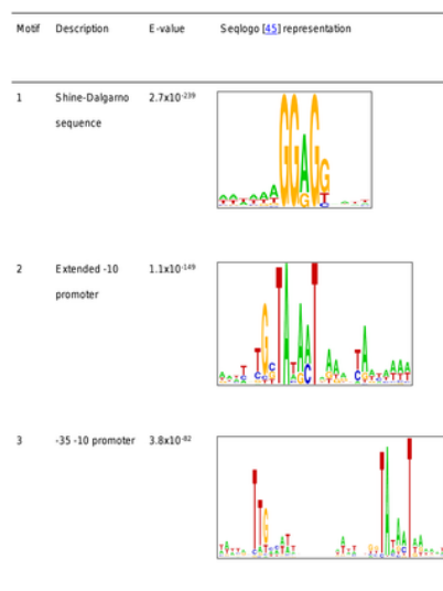
Figure 1. Highly conserved motifs.
