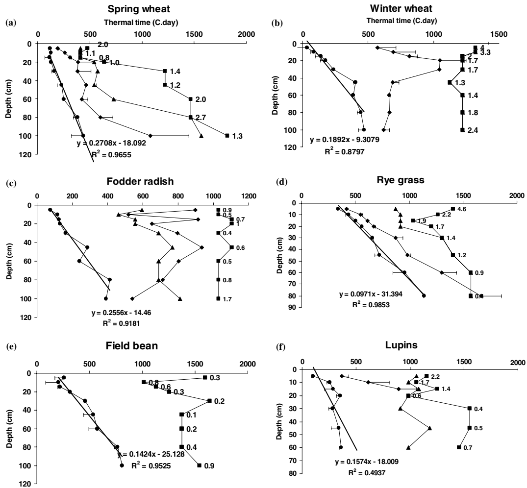
Figure 4. Thermal time after planting at 'first roots visible' ( N_{r,z,0} , ●), at root number = 0.5 \text{ cm}^{-2} ( N_{r,z,0.5} , ◆), at end of linear phase of root number increase ( N_{r,z,el} , ▲) and at maximum root number observed ( N_{r,z,m} , ■) vs. depth for spring wheat (a), winter wheat (b), fodder radish (c), ryegrass (d), field bean (e) and lupins (f). The maximum root number has been indicated (in \text{cm}^{-2} ).
