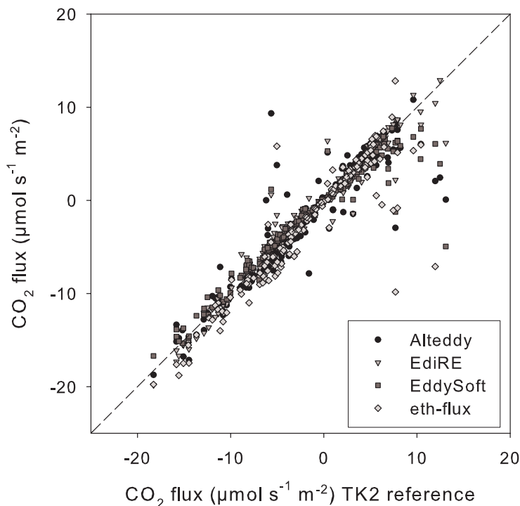
Fig. 4. CO 2 flux estimates from the site GRASATEM-2003 over grassland of 0.12 m canopy height (USA-1/LI-7500), calculated by the software packages Alteddy, EdiRE, EddySoft, eth-flux and TK2 as reference.
