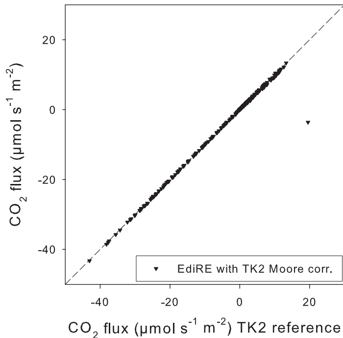
Fig. 3. CO 2 flux estimates computed from the same dataset as Fig. 2 using EdiRE, but replacing EdiRE's spectral correction by TK2's spectral correction.
