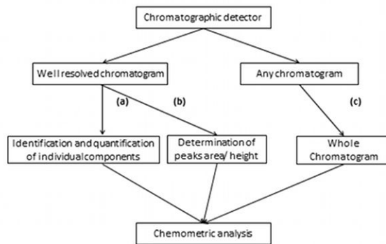
Figure 3. Schematic representation of the strategies to obtain multivariate dataset from a chromatogram for chemometric analysis.
