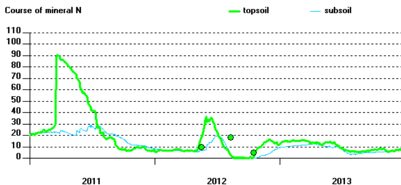
Figure 7: Course of soil mineral N. Green line is topsoil, 0-30 cm. Blue line is subsoil, 30-60 cm. Green dots are measurements in topsoil. Y-axis: \text{kg mineral N ha}^{-1}
