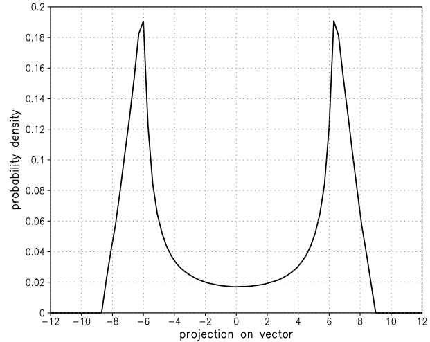
Fig 1. Probability density function of low-pass filtered time series of the projection onto the vector connecting the two regimes, for the LORENZ 63 model with standard parameter values.
