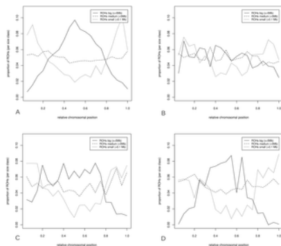
Figure 7. Distribution of ROHs over relative chromosomal position.
