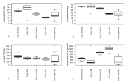
Figure 1. Summary statistics for genomic variation.
