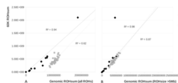
Figure 3. ROH size in pigs based on the 60K chip method and the re-sequencing method.
