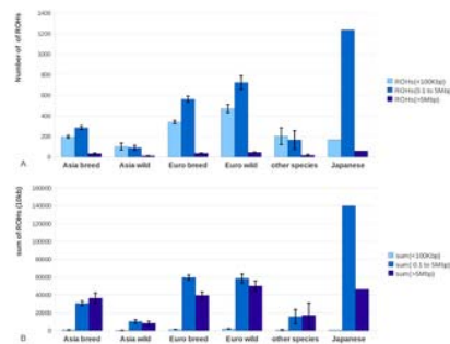
Figure 2. Total number of ROHs and proportion of the genome covered by ROHs.
