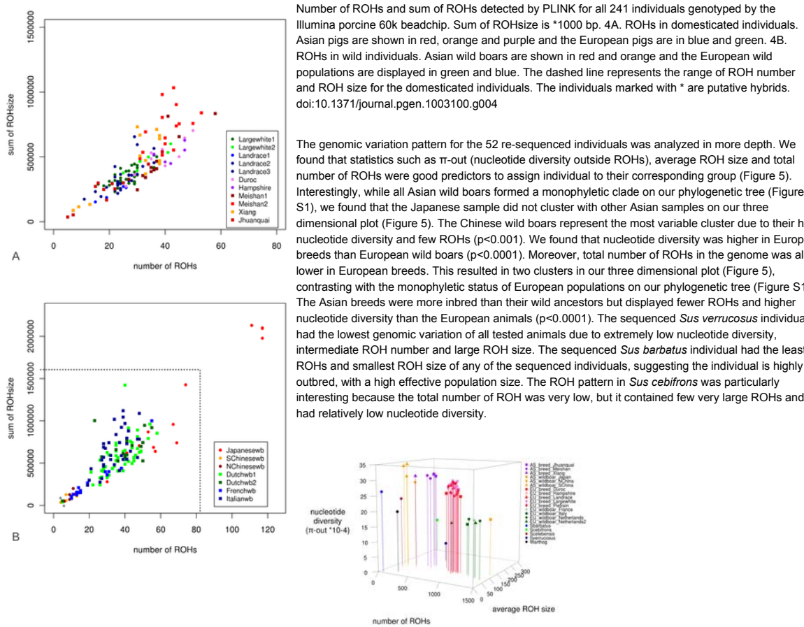
Figure 5. Three-point ROH statistics for all 52 sequenced individuals. On the x-axis, the number of ROHs in the genome per individual is plotted, the average ROH size (*10 4 bp) is displayed on the y-axis and the nucleotide diversity outside ROHs in a 10 kb window 'nucleotide diversity ( \pi -out *10 -4 )' on the z-axis. Coloration is based on relatedness and geography, with individuals from the same populations having the same color. doi:10.1371/journal.pgen.1003100.g005
