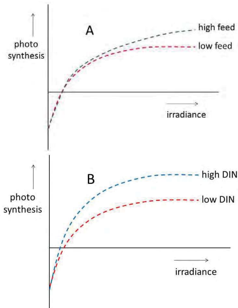
Fig. 10. Schematic representation of the findings of Houllbrèque et al. (2004) on the effects of feeding on photosynthesis in Stylophora pistillata (A) and the findings of Marubini & Davies (1996) on the effects of DIN enrichment on photosynthesis in Montastrea annularis and Porites porites (B).
