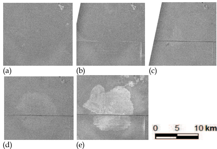
Fig. 5. JERS-1 SAR time series of the collapse of the peat dome in Kahiya: (a) 12 Jul 1995; (b) 19 Mar 1997; (c) 11 Sep 1997; (d) 25 Oct 1997; (e) 21 Jan 1998.
