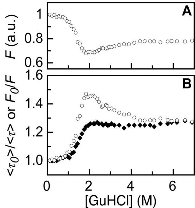
Figure 7. Tracking of changes in static and dynamic quenching of A488 fluorescence upon folding of A488-apoflavodoxin. (A) Denaturant dependence of A488 fluorescence F . A488 is excited at its denaturant-dependent fluorescence excitation maximum and A488 fluorescence is recorded at its denaturant-dependent fluorescence emission maximum. (B) Denaturant dependence of F_0/F (open dots) and \langle \tau_0 \rangle / \langle \tau \rangle (filled diamonds), calculated from the data in panel (A) and Fig. 5B, respectively. doi:10.1371/journal.pone.0046838.g007
