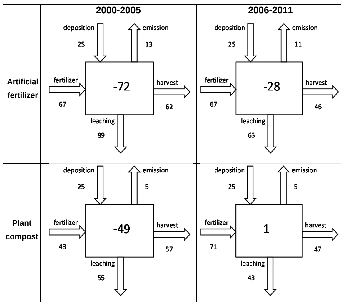
Figure 9: Nitrogen balances for the treatments artificial fertilizer and plant compost. All units are \text{kg ha}^{-1} \text{ year}^{-1} . Within the square: change in soil nitrogen. Emission: sum of denitrification and volatilization.
