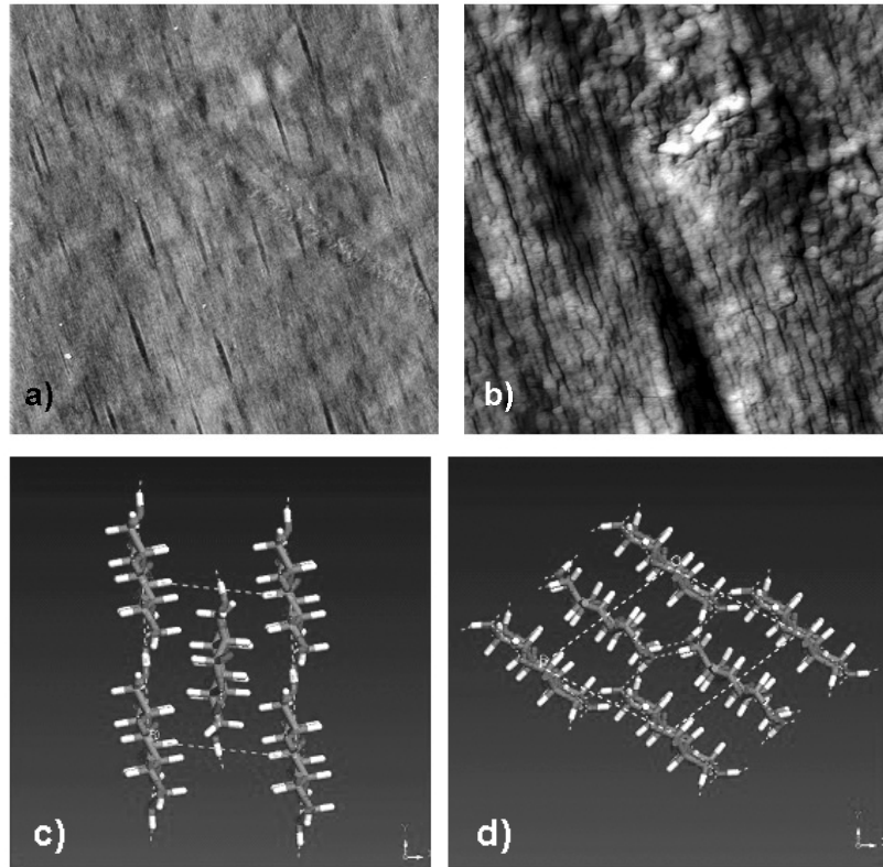
Figure 2.2: Images of (a) cellulose I and (b) cellulose II specimen. Projections of the 3d structure of (c) cellulose Ib and (d) cellulose II
