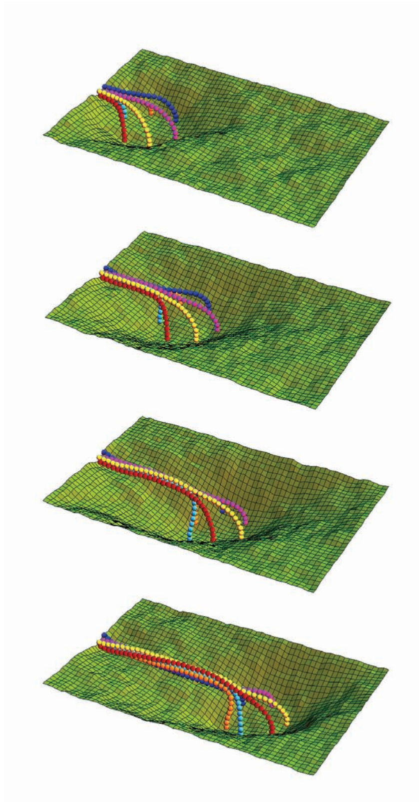
Figure 4.11: Snapshots at four different time points in a stochastic simulation of the motion of a six filament CSC. Note the rotation of the complex, induced by the helical nature of the crystalline arrangement in the CMF.
