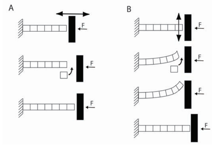
Figure 4.4: The two models for BPR: (a) rigid filaments and (b) semi-flexible filaments
