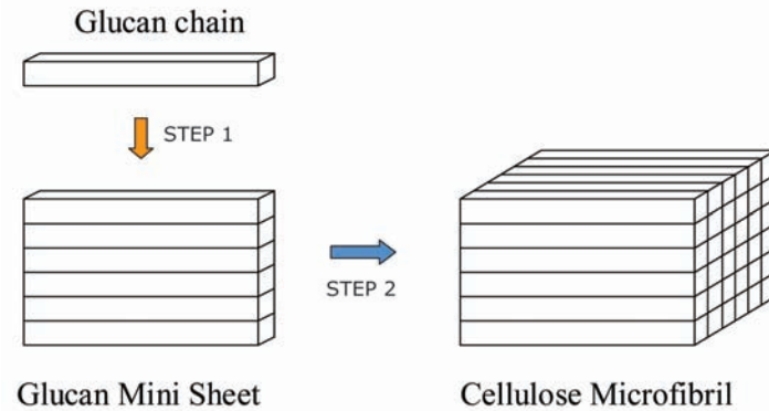
Figure 2.4: Scheme for the two-step crystallization process of the CMF: first, glucan chain coalesce in a monomolecular layer via Van der Waals forces; then the glucan sheets crystallize together through Hydrogen bonding to form a CMF.
