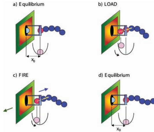
Figure 6.15: The Load and Fire mechanism
