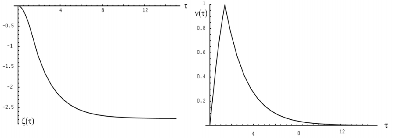
Figure 5.13: v(t) and \zeta(t) for the Poissonian case
