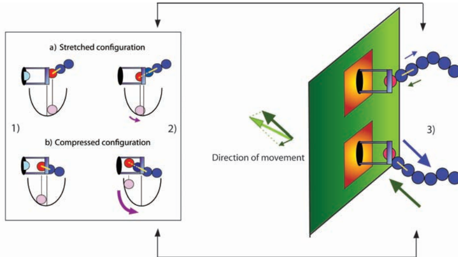
Figure 6.16: The final direction of motion of the bacterium depends on the magnitude and the direction of the pushing forces exerted by the filaments
