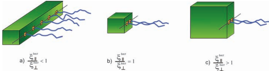
Figure 6.13: Possible shapes of the 3d-cuboidal body depending on the ratio on the drag coefficients
