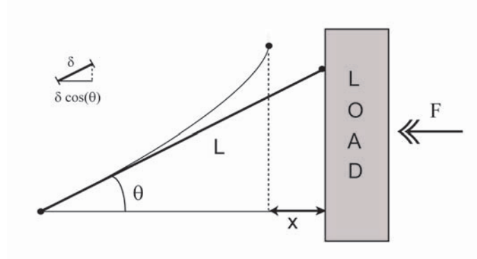
Figure 4.6: Details of BPR for semiflexible filaments
