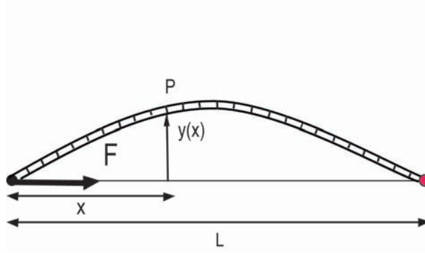
Figure 6.8: Euler buckling instability
