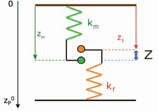
Figure 4.9: The effective model of two coupled springs the analytical model maps onto.
