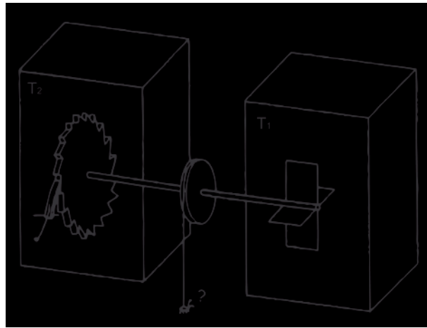
Figure 7.1: The Feynman's Brownian Ratchet
