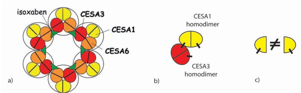
Figure 3.6: (a) Model for CESAs interactions in primary cell wall. (b) Interactions between CESA1 and CESA3 homodimers. (c) Interactions between two CESA1 subunits
