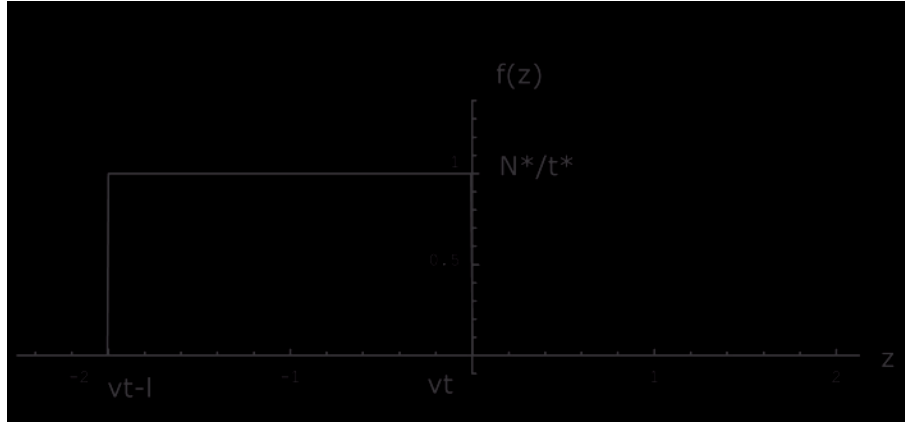
Figure 5.7: Square wave ID (birth rate function for \gamma = 0 )
