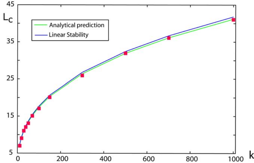
Figure 6.11: Theoretical (Eqs. 6.16 and 6.21 ) versus simulations results
