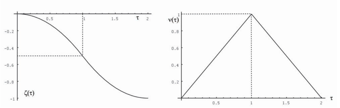
Figure 5.8: \zeta(\tau) and v(\tau) : the original helicoidal solution
