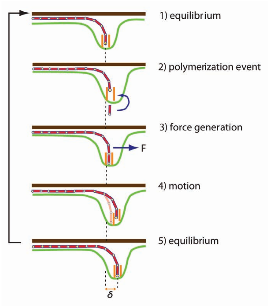
Figure 4.7: Schematic representation of the mechanical cycle in our model of CSC propulsion, illustrated for the case of a single CMF. From top to bottom: Step 1: the filament and the membrane are in thermal equilibrium. Step 2: due to fluctuations of the filament and/or the membrane, a gap of sufficient size is opened allowing a new monomer to be added to the filament. Step 3: the increase in length of the filament causes an accumulation of elastic energy in the system, which generates a force on the tip of the filament. Step 4: the accumulated energy is released in a unidirectional motion of the tip of the filament, which is attached to the CSC. Step 5: the filament has effectively advanced by one monomer unit and equilibrium is restored, allowing the cycle to repeat itself.
