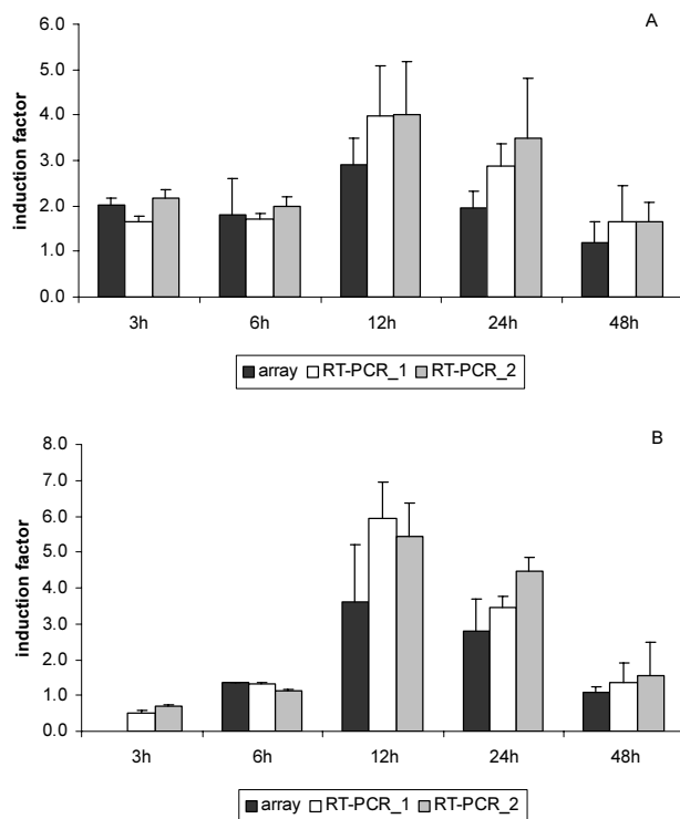
Figure 5 AKR1C1 gene expression changes in response to curcumin [A: low concentration, B: high concentration], measured with cDNA microarray (black bars), and measured by real time RT-PCR normalized to beta-actin expression (white bars) or to GAPDH expression (grey bars). Expression is plotted as induction factors (level in treated cells compared to untreated cells) (mean \pm standard deviation).
