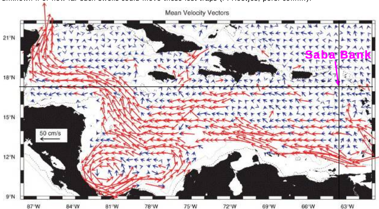
Figure 11. Mean current velocity grouped into ½-degree by ½-degree bins. The strong Caribbean Current is shown by red arrows (>25 cm/second) and the location of the Saba Bank is marked at the intersection of the black lines at 17°25' N and 63°30' W (Adapted from Richardson 2005).
