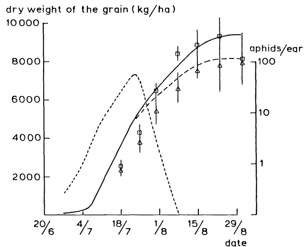
Fig. 1. Simulated (—) and measured (□) dry weight of the grain in the absence of aphids, simulated (---) and measured (△) dry weight of the grain in the presence of aphids and the aphid population (----), as a function of time.
