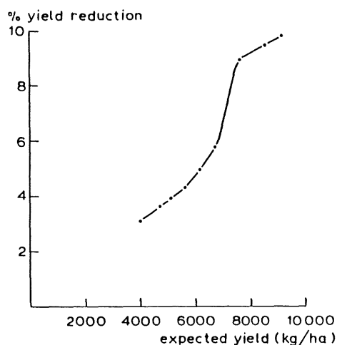
Fig. 3. Percentage yield reduction according to the simulation model at an aphid intensity of 490 aphid-days as a function of the yield level in the absence of aphids.
