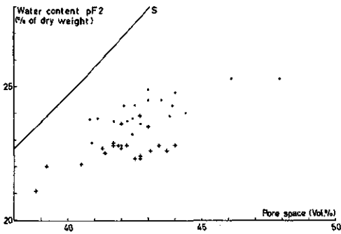
Fig. 7 Relation between water content at pF2 and pore space on an untilled plot on a heavy river clay (Randwijk), showing decrease in water content at pF2 during winter. • autumn 1967; + spring 1968.
