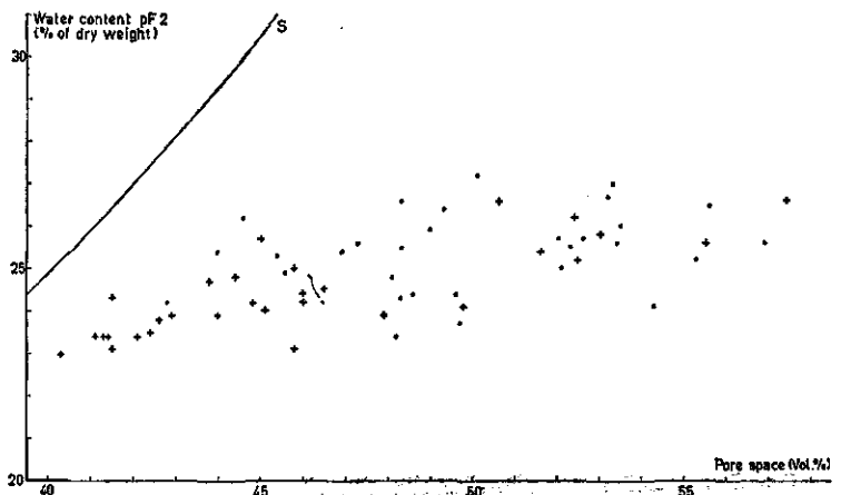
Fig. 4 Relation between water content at pF2 and pore space on a tilled and an untilled plot on a heavy marine silt (Westmaas). Spring barley after potato. Statistical character of difference between treatments; 15 September 1969. • ploughing; + zero-tillage.
