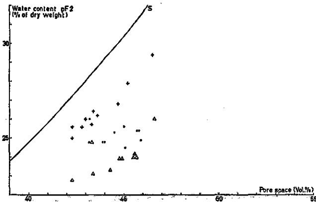
Fig. 9 Relation between water content at pF2 and pore space on an untilled plot on a heavy river clay (Randwijk). Changes in water content at pF2 are parallel to Fig. 8. • autumn 1968; + spring 1969; Δ autumn 1969.
