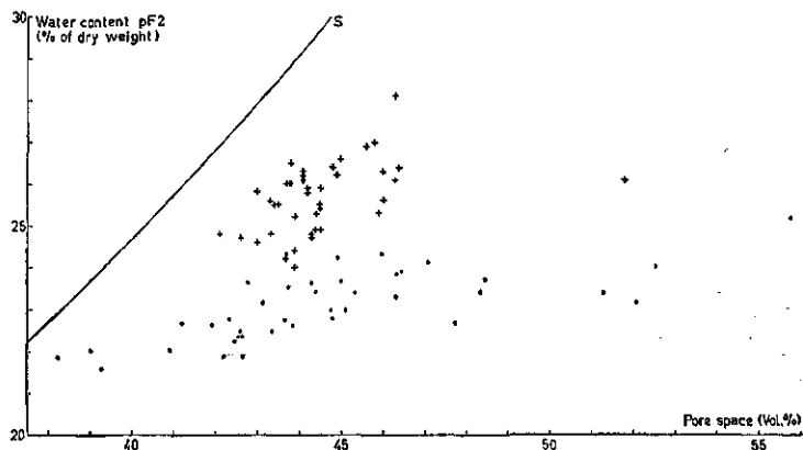
Fig. 6 Relation between water content at pF2 and pore space on a tilled and an untilled plot on a heavy river clay (Randwijk), showing decrease in pore space and increase in water content at pF2 after one year zero-tillage. • spring 1964; + spring 1965.
