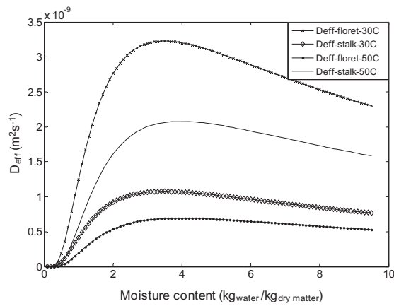
Fig. 3. Effective diffusion coefficients for broccoli florets and broccoli stalks at 30°C and 50°C
