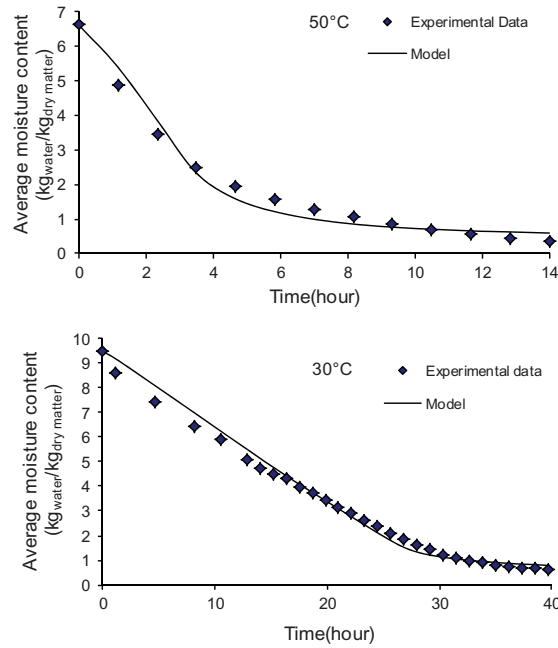
Fig. 2. Measured and estimated drying profiles: Top: at 50°C, bottom at 30°C
