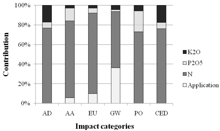
Fig. 6. Fertilizers contribution to impact categories for a glasshouse tomato crop in the Netherlands. Impact categories: AD, abiotic depletion; AA, air acidification; EU, eutrophication; GW, global warming; PO, photochemical oxidation; CED, cumulative energy demand.
