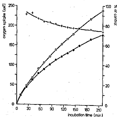
FIG. 6.1. Effect of 10^{-4} M pyrazophos on oxygen uptake by Sphaerotheca fuliginea conidia. Concentration of conidia: 19.6 \times 10^6 /ml. Control (○—○); pyrazophos (●—●); oxygen uptake in the presence of pyrazophos as % of control (+—+).
