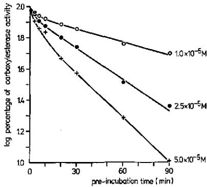
FIG. 4.5. Carboxylesterase activity in a cell-free extract of Sphaerotheca fuliginea conidia in relation to time of pre-incubation of a mixture of extract and pyrazophos, at concentrations of pyrazophos as indicated in figure. After pre-incubation, 0.2 ml of the mixture was diluted with 5 ml 3.12 \times 10^{-4} M NA in 0.04 M phosphate buffer pH 7. Residual esterase activity was determined by measuring the \alpha -naphthol-diazoblu complex formation in the incubation mixture after 20 min of incubation.
