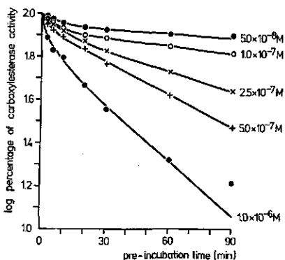
Fig. 4.6. Carboxylesterase activity in a cell-free extract of Sphaerotheca fuliginea conidia in relation to time of pre-incubation of a mixture of extract and PO-pyrazophos, at concentrations of PO-pyrazophos as indicated in figure. After pre-incubation, 0.2 ml of the mixture was diluted with 5 ml 3.12 \times 10^{-4} M NA in 0.04 M phosphate buffer pH 7. Residual esterase activity was determined by measuring the \alpha -naphthol-diazoblu complex formation in the incubation mixture after 20 min of incubation.
