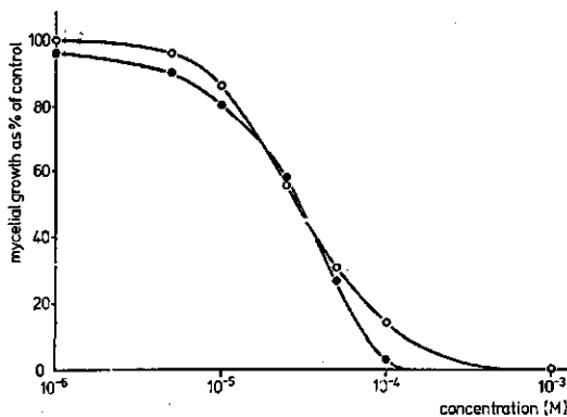
FIG. 3.5. Effect of Hinosan (●-●) and Kitazin (○-○) on mycelial growth of Pyricularia oryzae in vitro on Gly agar.
