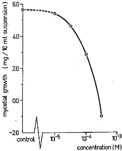
FIG. 8.3. Mycelial growth of Pyricularia oryzae in liquid Gly medium in 0.05 M McIlvaine buffer pH 4.0 in relation to concentration of PP. Incubation time: 2 hours. Initial dry weight 34.8 mg/10 ml suspension.
