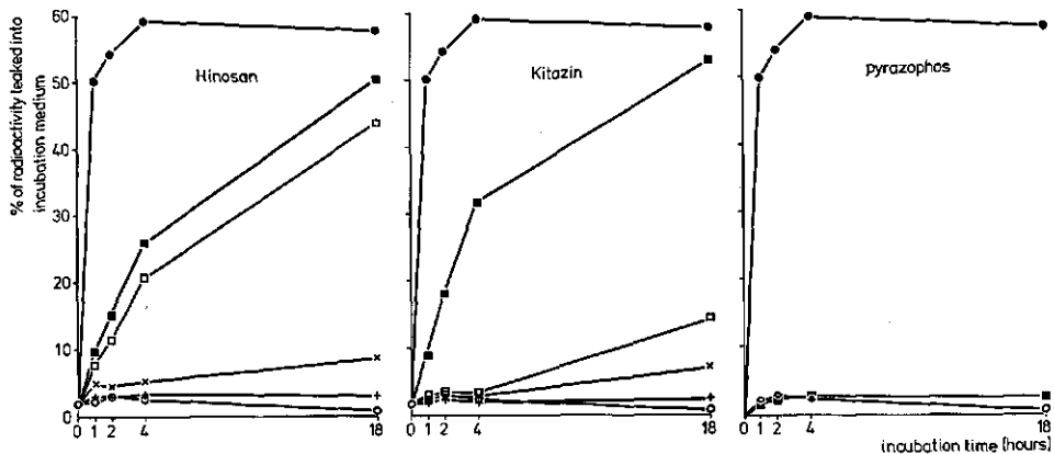
FIG. 5.3. Effect of Hinosan, Kitazin, pyrazophos and chloroform on leakage of ^{32}\text{P} -orthophosphate from mycelial cells of Pyricularia oryzae into incubation medium. Control (○—○), Hinosan, Kitazin or pyrazophos concentrations 3.2 \times 10^{-5} M (+—+), 10^{-4} M (×—×), 3.2 \times 10^{-4} M (□—□), and 10^{-3} M (■—■), and chloroform (1%) (●—●).
