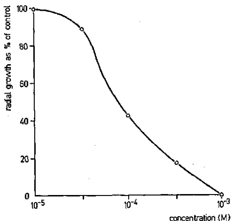
FIG. 8.2. Radial growth of Pyricularia oryzae on Gly-agar in 0.05 M McIlvaine buffer pH 4.0 in relation to concentration of PP.
