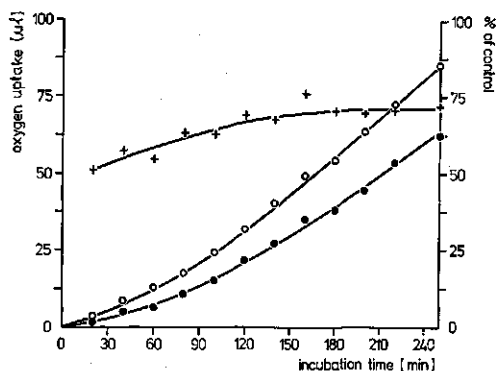
FIG. 6.2. Effect of 10^{-3} M pyrazophos on oxygen uptake by mycelium of Pyricularia oryzae in Gly medium. Initial dry weight of mycelial suspension 0.4 mg/ml. Control (○—○) pyrazophos (●—●); oxygen uptake in the presence of pyrazophos as % of control (+—+).
