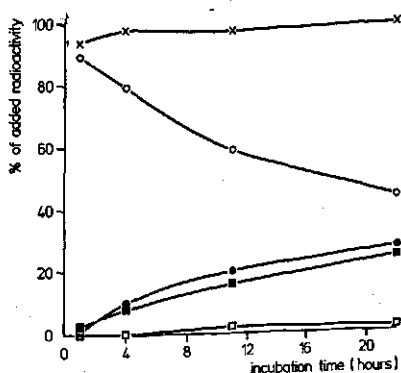
FIG. 7.2. Distribution of added radioactivity in ^{14}\text{C} -pyrazophos (○—○), ^{14}\text{C} -PO-pyrazophos (●—●), ^{14}\text{C} -PP (□—□) and non-identified ^{14}\text{C} -labelled metabolites (■—■) in liquid cultures of Pyricularia oryzae in Gly medium in relation to time. Recovery of added radioactivity (×—×); cultures incubated with 10^{-5} M pyrazophos (spec. act. c. 0.36 mCi/mmole).
