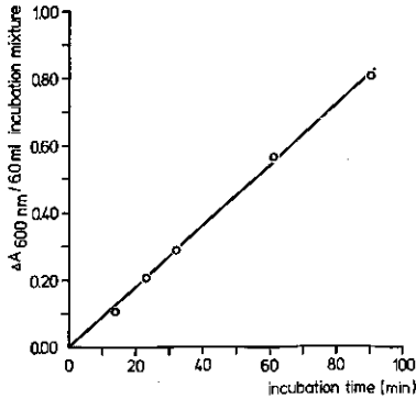
FIG. 4.2. NA hydrolysis by esterases in a cell-free extract of Sphaerotheca fuliginea conidia in relation to incubation time. Assay medium: 6 ml of 2.5 \times 10^{-4} M NA in 0.04 M phosphate buffer pH 7, containing a fixed amount of cell-free extract; degree of hydrolysis measured as \alpha -naphthol-diazoblu complex formation ( \Delta A_{600nm} ) after various incubation times.
