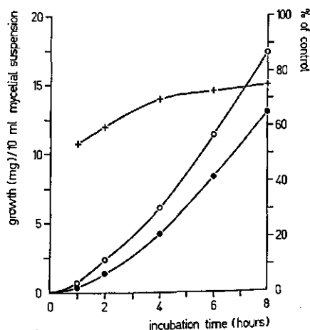
FIG. 6.3. Effect of 10^{-3} M pyrazophos on mycelial growth of Pyricularia oryzae in liquid Gly medium. Initial dry weight of mycelial suspension 1.5 mg/ml. Control (○—○); pyrazophos (●—●); mycelial growth in the presence of pyrazophos as % of control (+—+).
