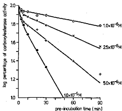
FIG. 4.7. Carboxylesterase activity in a cell-free extract of Sphaerotheca fuliginea conidia in relation to time of pre-incubation of a mixture of extract and paraoxon, at concentrations of paraoxon as indicated in figure. After pre-incubation, 0.2 ml of the mixture was diluted with 5 ml 3.12 \times 10^{-4} M NA in 0.04 M phosphate buffer pH 7. Residual esterase activity was determined by measuring the \alpha -naphthol-diazoblu complex formation in the incubation mixture after 20 min of incubation.
