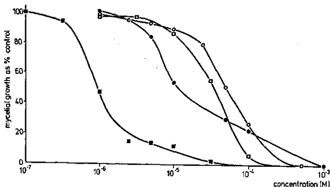
FIG. 3.4. Effect of pyrazophos and PO-pyrazophos on mycelial growth of Pyricularia oryzae in vitro on Gly agar and in shake cultures of the same composition without agar. Agar medium with pyrazophos: (●—●) and PO-pyrazophos: (○—○); shake culture with pyrazophos: (■—■) and PO-pyrazophos: (□—□).
