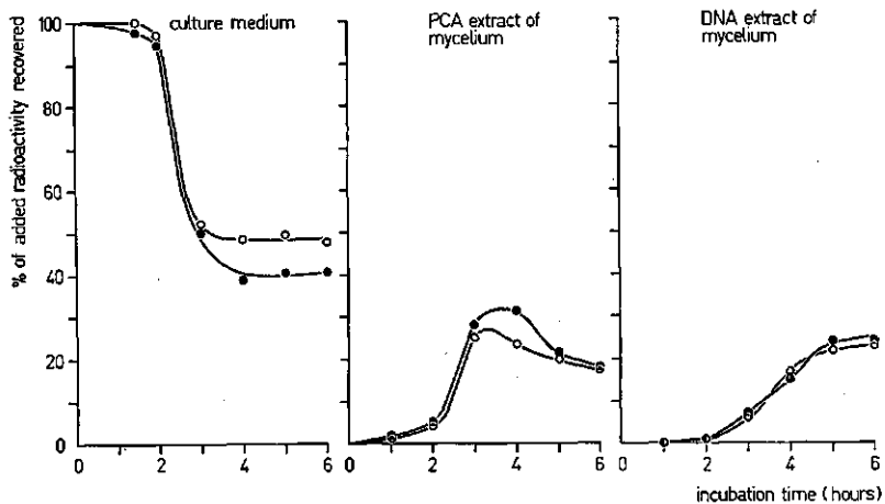
FIG. 6.4. Effect of 10^{-3} M pyrazophos on incorporation of ^{14}\text{C} -thy by mycelium of Pyricularia oryzae . Pyrazophos and ^{14}\text{C} -thy were added simultaneously to the mycelial suspension. Control (○—○); pyrazophos (●—●).
