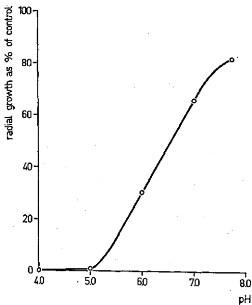
FIG. 8.1. Effect of pH on inhibition of radial growth of Pyricularia oryzae by 10^{-3} M PP. The fungus was grown on Gly-agar, prepared in 0.05 M McIlvaine buffer (pH 4.0, 5.0 and 6.0) or 0.05 M phosphate buffer (pH 7.0 and 8.0).
