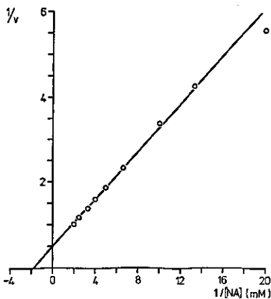
FIG. 4.3. Esterase activity ( v ) in a cell-free extract of Sphaerotheca fuliginea conidia in relation to NA concentration. Assay medium: 6 ml of 0.5 – 5.0 \times 10^{-4} M NA in 0.04 M phosphate buffer pH 7, containing a fixed amount of cell-free extract; v = \alpha -naphthol-diazoblu complex formation in incubation mixture, expressed as \Delta A_{600nm} after 20 min of incubation.
