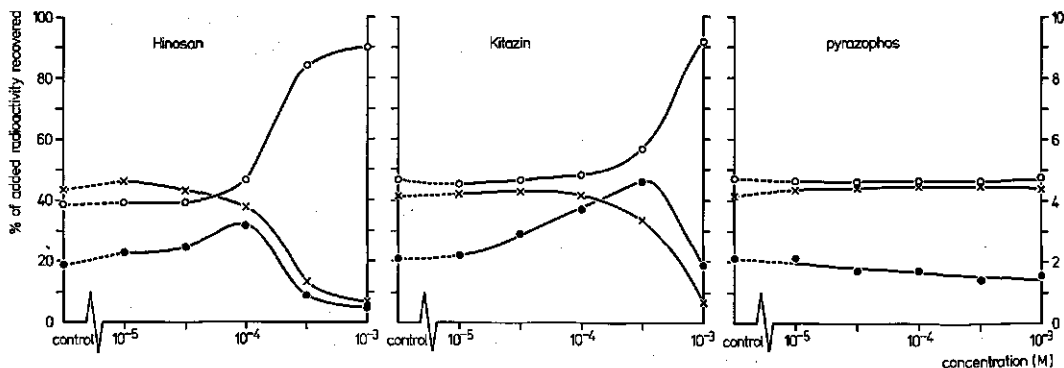
FIG. 5.1. Effects of Hinosan, Kitazin and pyrazophos on incorporation of ^{14}\text{C} -glucosamine by mycelium of Pyricularia oryzae . Percentages of added radioactivity recovered in incubation media (O—O), TCA-extracts of mycelium (●—●) and mycelial residues (x—x). Percentages of radioactivity recovered in TCA-extracts have been expressed on a 10 \times enlarged scale.
