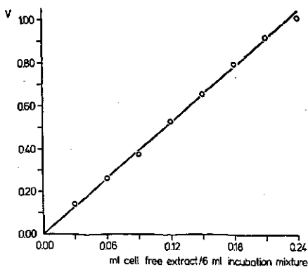
Fig. 4.1. Esterase activity (v) in relation to concentration of a cell-free extract of Sphaerotheca fuliginea conidia. Assay medium: 6 ml of 2.5 \times 10^{-4} M NA in 0.04 M phosphate buffer pH 7, containing various amounts of cell-free extracts; v = \alpha -naphthol-diazoblu complex formation in incubation mixture expressed as \Delta A_{600nm} after 20 min of incubation.
