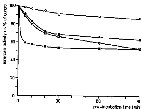
FIG. 4.8. Esterase activity of Sphaerotheca fuliginea conidia in relation to time of pre-incubation of a conidial suspension with inhibitor; final concentrations of inhibitors: 10^{-5} (○—○) and 10^{-4} M (●—●) pyrazophos or 10^{-6} (□—□) and 10^{-5} M (■—■) PO-pyrazophos. After pre-incubation, 0.4 ml of the mixture was diluted with 10 ml 3.12 \times 10^{-4} M NA in 0.04 M phosphate buffer pH 7. Residual esterase activity was determined by measuring the \alpha -naphthol-diazoblue complex formation in the incubation mixture after 20 min of incubation.
