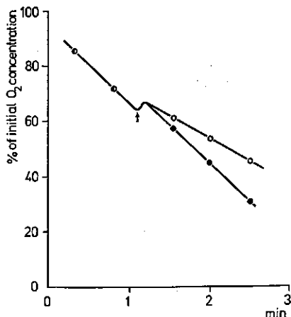
FIG. 9.1. Effect of 5 \times 10^{-4} M PP on the rate of oxygen uptake of Pyricularia oryzae . The arrow indicates the time when a control amount of acetone (●-●) or PP, dissolved in acetone, (○-○) were added.
