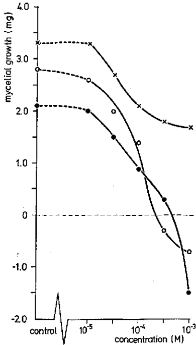
FIG. 5.2. Effect of Hinosan (○—○), Kitazin (●—●) and pyrazophos (×—×) on mycelial growth of Pyricularia oryzae during a 2 hour incubation period. Initial dry weight 19.2, 9.6 and 11.4 mg per 10 ml mycelial suspensions, respectively.
