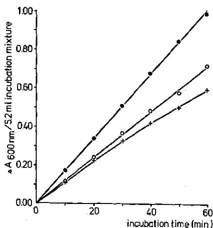
FIG. 4.4. NA hydrolysis by esterases in a cell-free extract of Sphaerotheca fuliginea conidia in relation to incubation time, after 3 min pre-incubation of 0.1 ml of extract with 0.1 ml of inhibitor solution, resulting in final concentrations of 5 \times 10^{-5} M pyrazophos (○—○), 10^{-6} M PO-pyrazophos (●—●), and 5 \times 10^{-5} M paraoxon (+—+). After pre-incubation, the mixture was diluted with 5 ml 3.12 \times 10^{-4} M NA in 0.04 M phosphate buffer pH 7; degree of hydrolysis measured as \alpha -naphthol-diazoblu complex formation ( \Delta A_{600nm} ) after various incubation times.
