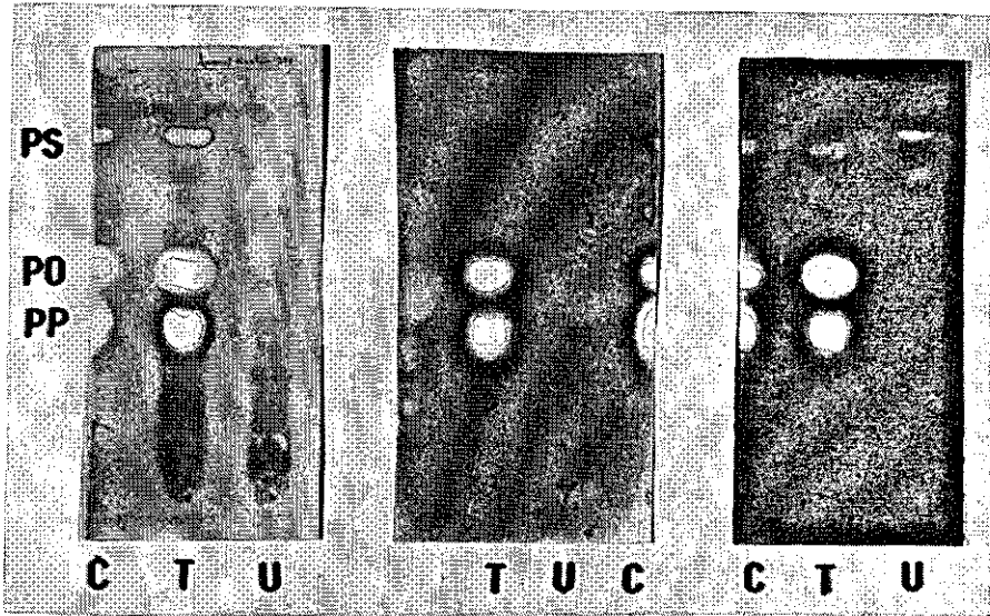
FIG. 7.4. TLC-bioassays of toluene extracts of culture media of Pyricularia oryzae , incubated for 22 hours with 10^{-3} M pyrazophos and subsequently acidified with PCA to a final concentration of 0.5%: Solvent: benzene/acetone 3:1. Test fungi: Fusarium culmorum (left), Ascochyta pisi (middle), Cladosporium cucumerinum (right). C: references of pyrazophos (PS), PO-pyrazophos (PO) and PP; T and U: extracts of mycelium with and without 10^{-3} M pyrazophos, respectively.
