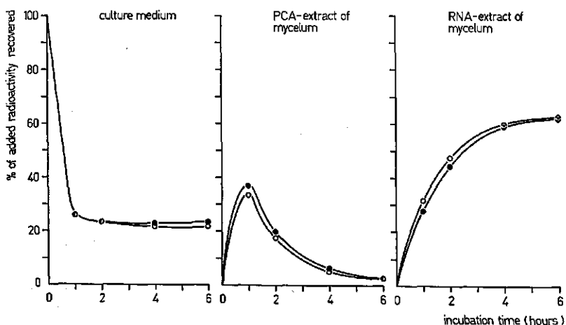
FIG. 6.5. Effect of 10^{-3} M pyrazophos on incorporation of ^{14}\text{C} -ur by mycelium of Pyricularia oryzae . Pyrazophos and ^{14}\text{C} -ur were added simultaneously to the mycelial suspension. Control (○—○); pyrazophos (●—●).
