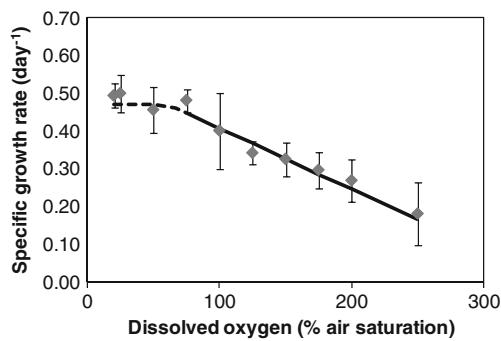
Fig. 3 Effects of oxygen concentration on the specific growth rate ( \text{day}^{-1} ) of Nannochloropsis sp. at an irradiance of 100 \mu\text{mol photons m}^{-2} \text{s}^{-1}
