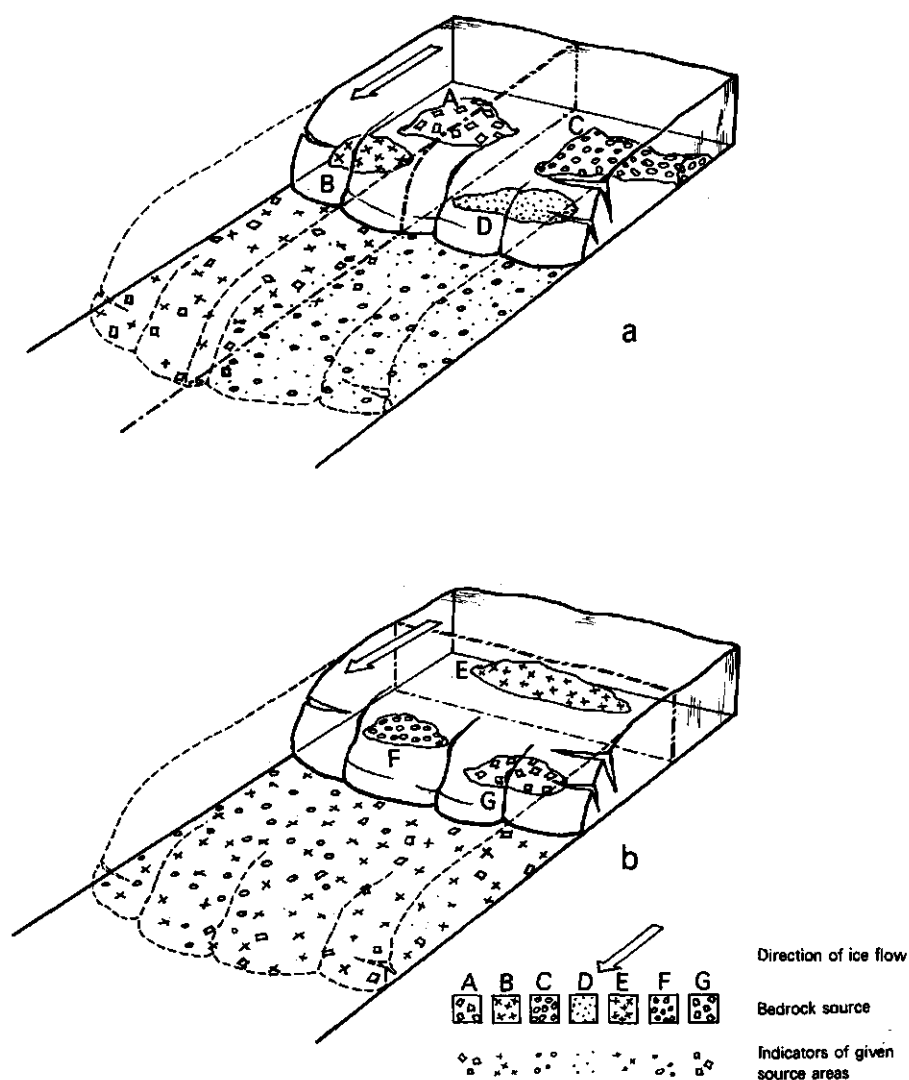
Fig. 1. Schematic representations of segments of an ice sheet. Source areas separated by lines parallel (a) and transverse (b) to the flow direction.
