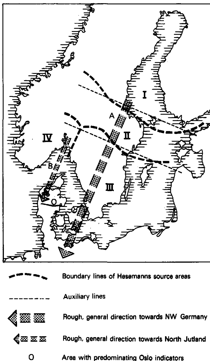
Fig. 2. Generalized mean ice stream directions tentatively reconstructed on the basis of the trends shown by the boundary lines of Hesemann's source areas.
