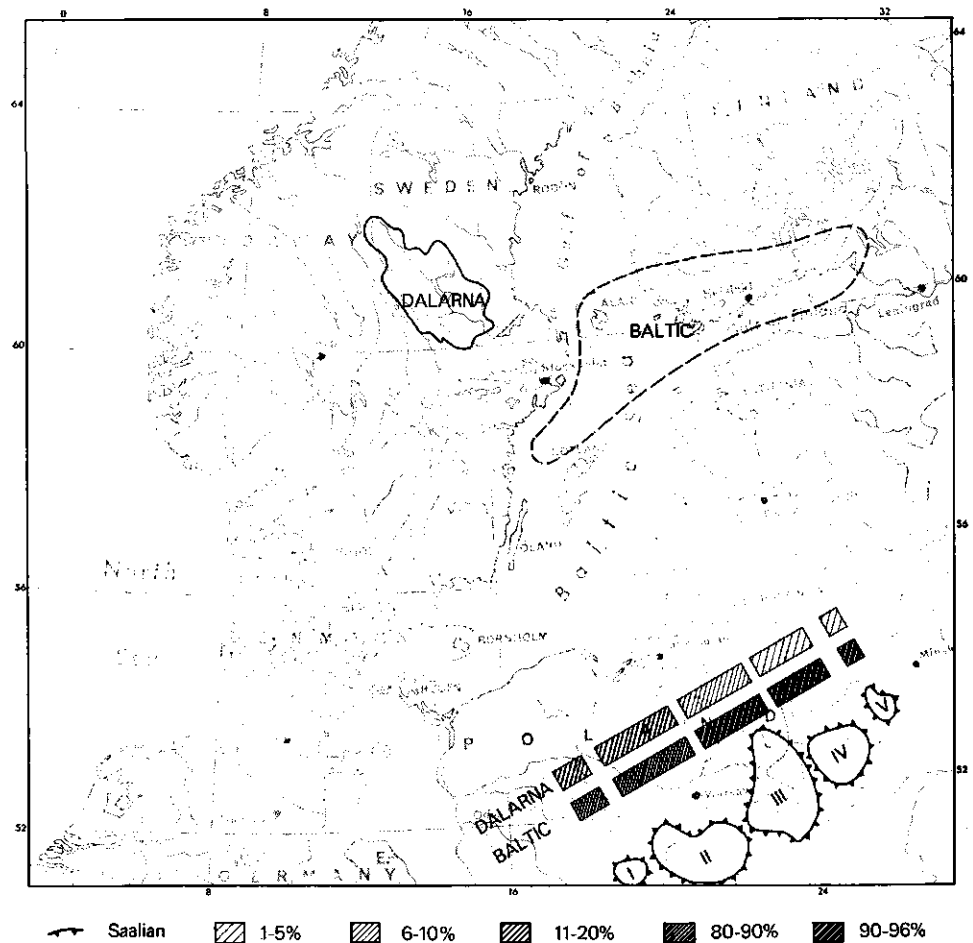
Fig. 18. The eastward trend of the Saalian indicator distribution in Poland and White Russia. For Roman numerals, see Table 9.
