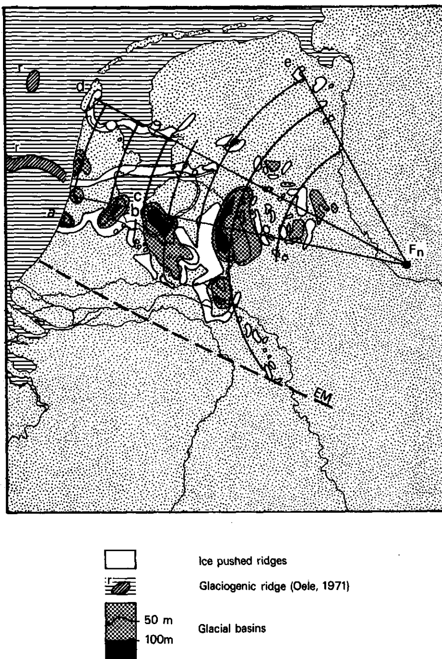
Fig. 40. The pattern of the Saalian morphology in The Netherlands in relation to circular tracts about F_n . Saalian after retreat of inland ice from Zagwijn (1974). a, b, c, d, e: Saalian ice front phases according to Maarleveld (1958, 1960) and ter Wee (1962). EM: part of the confocal ellipse to which the maximum of the Saalian in The Netherlands approaches.
