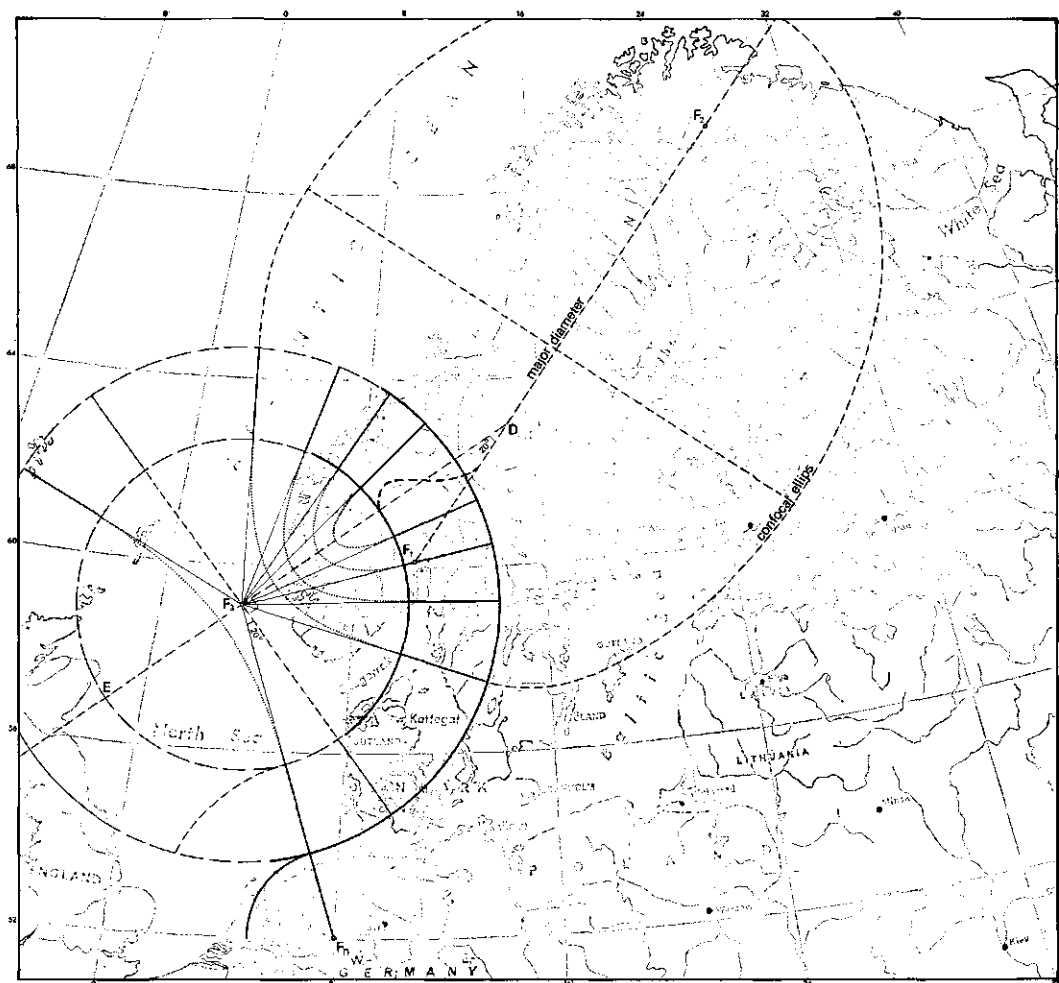
Fig. 41. Morainic contours on the inside of the circular zone, constructed by symmetry operations. For explanation, see text.
