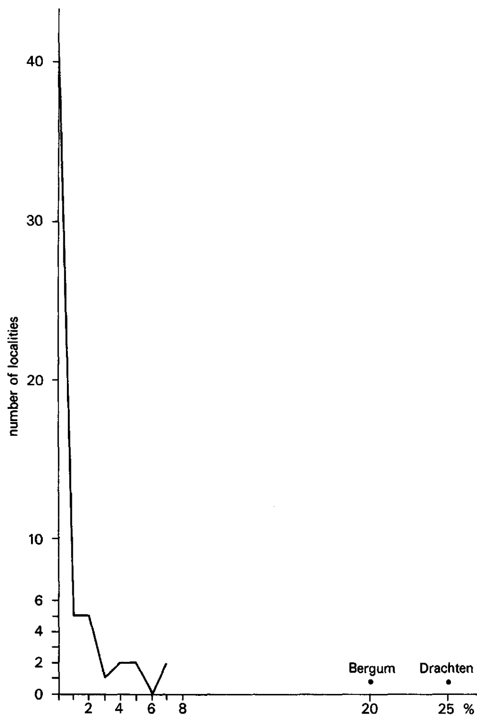
Fig. 14. Distribution of the Oslo indicators in The Netherlands.
