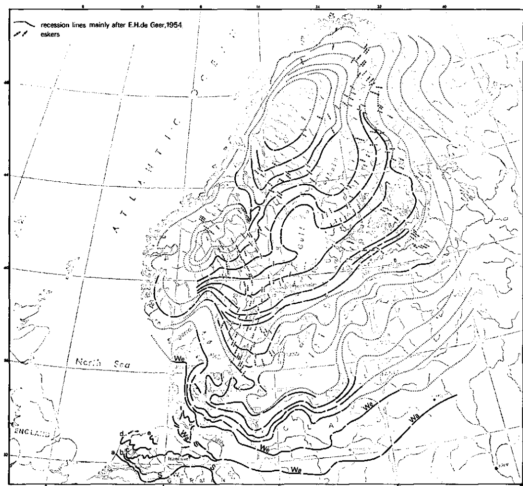
Fig. 25. Recession lines and maximum extension of ice sheets in relation to esker pattern. For further explanation, see text.
