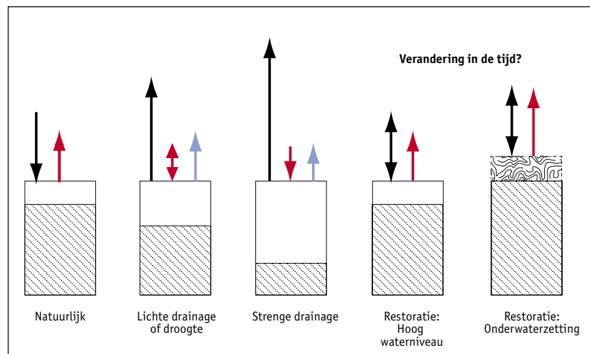
Figure 1 relative magnitudes of net exchange of CO 2 (black arrow), CH 4 (red arrow) and N 2 O (blue arrow) in peat lands with different management regimes and ground water tables. Lined areas symbolize saturated part of the profile and waves in last panel indicate flooding (based on Drösler et al. , 2008).
