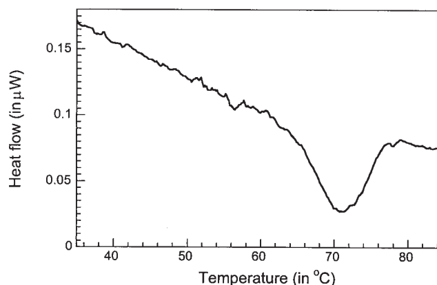
FIGURE 6 DSC thermogram of the F_c fragment (3.8 mg/ml) in a 0.1 M phosphate buffer, pH 8.1. Heating rate 0.5°C/min.
