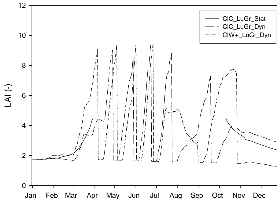
Fig. 8. Simulated Leaf Area Index of grassland in evaluation point EP1 (Fig. 4), for three of the variants (Table 3):
