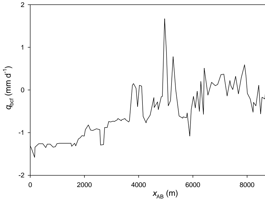
Fig. 7. Simulated net groundwater flux (Darcy flow, “BCF” in MODFLOW) for 2003 (time average), for the cross-section AB in Fig. 4.
