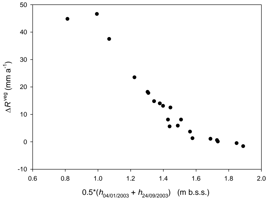
Fig. 11. Relationship between the mean groundwater level on day 4 January 2003 (day 4) and 24 September 2003 (day 264) and the difference between the recharge that is simulated for the W^+ scenario with dynamic and static vegetation models, with \Delta R^{\text{veg}} = R_{\text{dyn}} - R_{\text{stat}} ( \text{mm a}^{-1} ).
