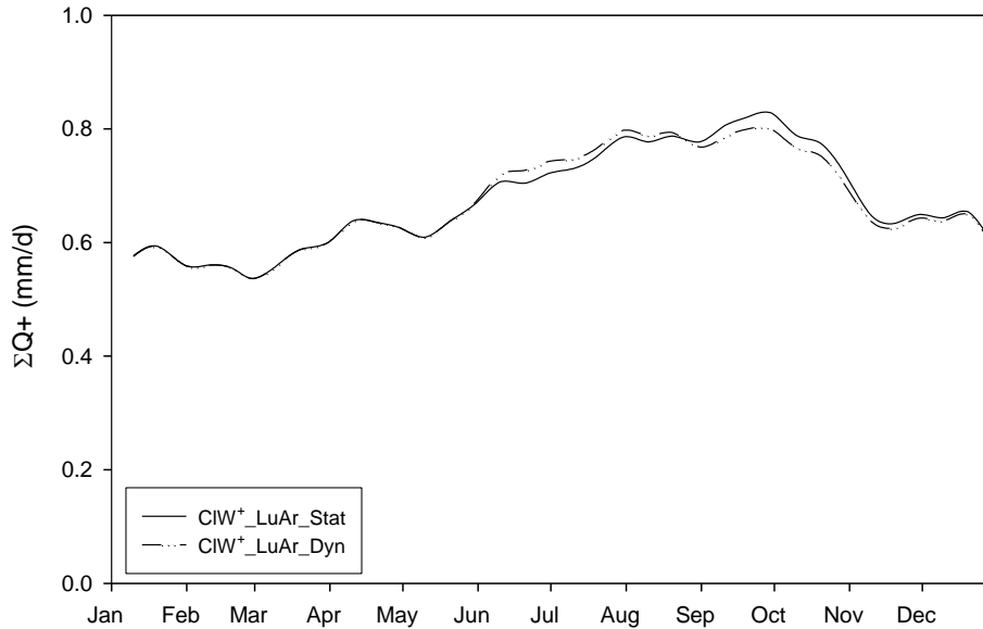
Fig. 13. Simulated total water demand, with static and dynamic vegetation models, for the W + scenario. The simulations are for the year 2063.
