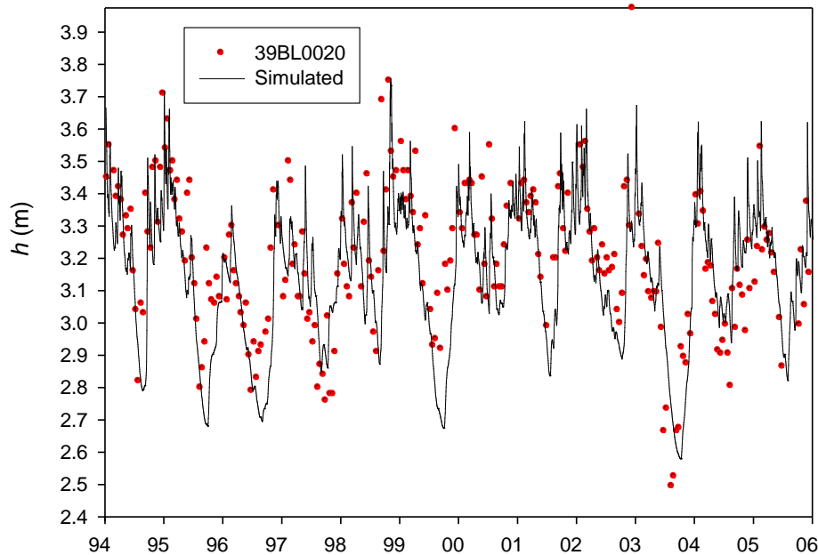
Fig. 5. Measured and simulated phreatic levels for the monitoring point 39BL0020 indicated in Fig. 4.
