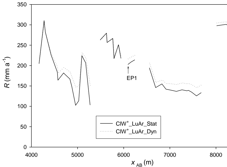
Fig. 10. Simulated recharge ( P - ET_a ) along the cross-section AB (Fig. 4), for the part that is in use by agriculture. The plot is for the arable land scenarios (“LuAr”), for the static/dynamic arable land simulations, for the W^+ climate scenario.
