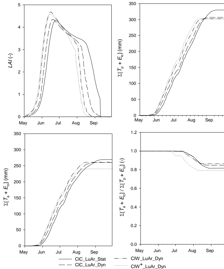
Fig. 9. Simulation results for arable land (potatoes) in evaluation point EP1 (Fig. 4), for four of the variants (Table 3): CIC - current climate, CIW/W + - scenarios, Stat/Dyn - static/dynamic vegetation model. The simulations are for the year 2003 (warm year, current climate) and 2063 (W/W + -scenario).
