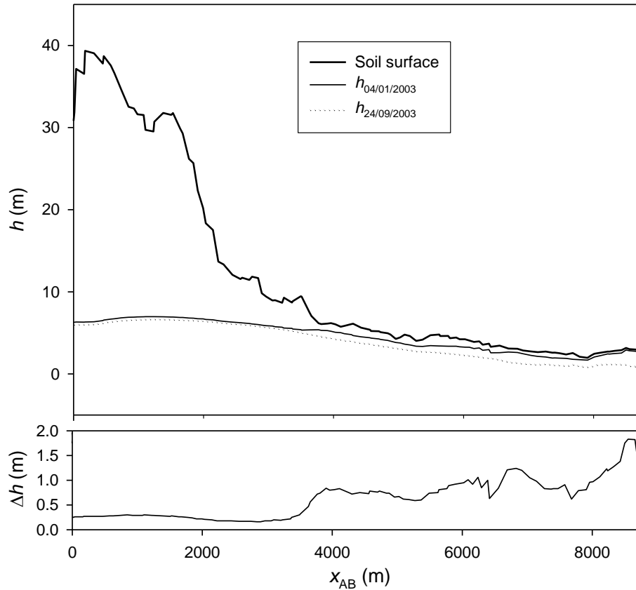
Fig. 6. Simulated groundwater level for 2003 (highest and lowest levels), for the cross-section AB in Fig. 4, and the groundwater level fluctuation \Delta h = h_{04/01/2003} - h_{24/09/2003} .
