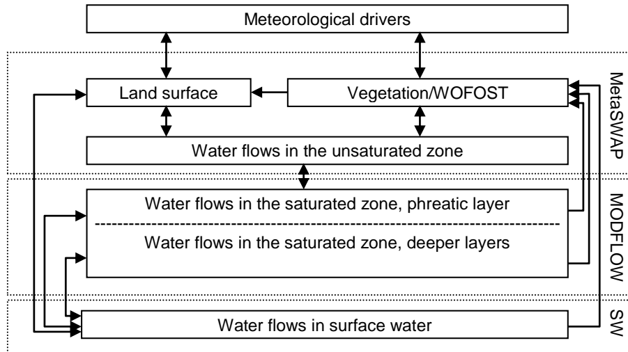
Fig. 1. Overview of SIMGRO modelling system.
