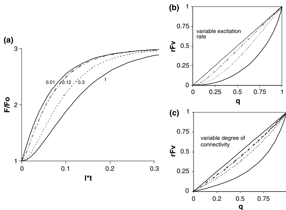
Fig. 2 (a) Accumulation of state y_2(t) = 1 - \frac{k_{s1}}{k_{s1} - k_L} e^{-k_L t} + \frac{k_L}{k_{s1} - k_L} e^{-k_{s1} t} (Eq. 3), representing the release of fluorescence quenching (expressed as F(t)/F_0 = 1 + nFv^{STF} \times y_2(t) (Eq. 8 with nFv^{STF} \sim 2 ) plotted as a function of incident energy I \times t ( I is incident light intensity) at variable excitation rates (intensities) k_L , relative to an assumed rate constant of donor side quenching release k_{s1} = 15 \text{ ms}^{-1} . k_L (= \alpha \times k_{s1}) was attenuated with factor \alpha = 1, 0.3, 0.12 , and 0.01 (curves from bottom to top). With \alpha = 1 ( I = 100\% ) the numbers on the I \times t -axis can be read in ms units. (b) The relative variable fluorescence yield rFv (= y_2(t)) plotted as a function of the fraction B(=q) of RCs with Q_A^- ('closed') with q = 1 - e^{-k_L t} (Eq. 5). Calculated curves (from bottom to top) are for \alpha = 1, 0.3, 0.1 , and
