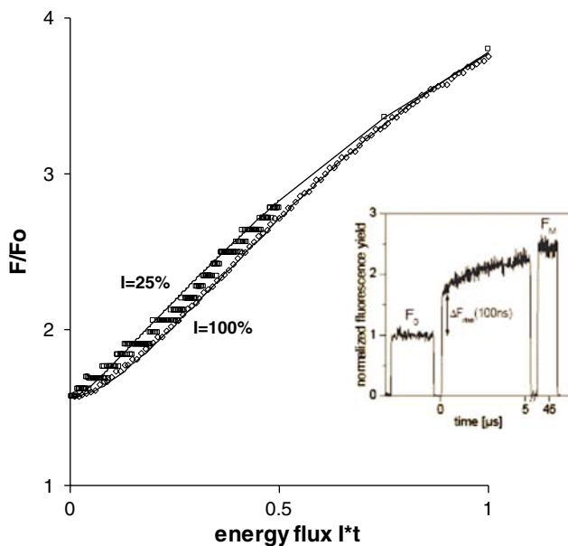
Fig. 6 Fluorescence increase (symbols) in dark-adapted Chenopodium chloroplasts ( 10 \mu\text{g chl/ml} ) in the presence of DCMU at 100% (lower curve) and at 25% of incident intensity ( I ) plotted as function of light flux I \times t . I \times t = 1 for full intensity corresponds with t = 1 ms, which means for I = 25\% with t = 4 ms. Solid lines are the fits of the experimental curves, calculated with TSTM and application of Eq. 10 (Hiraki et al. 2003; Vredenberg 2004). The figure shows that the sigmoidicity is less at a lower intensity (excitation rate k_L ). The right hand insert shows a laser flash induced increase in fluorescence in spinach chloroplasts, relative to F_0 , in the time range from 0–45 \mu\text{s} (reproduced from Fig. 28 in Steffen 2003). Note that in the laser flash the maximum fluorescence ( F_m^{\text{STF}} ) at 45 \mu\text{s} relative to F_0 is F_m^{\text{STF}}/F_0 \sim 2.4 , whereas in a 1 s MTF F_m^{\text{MTF}}/F_0 \sim 5 (see Fig. 4)
