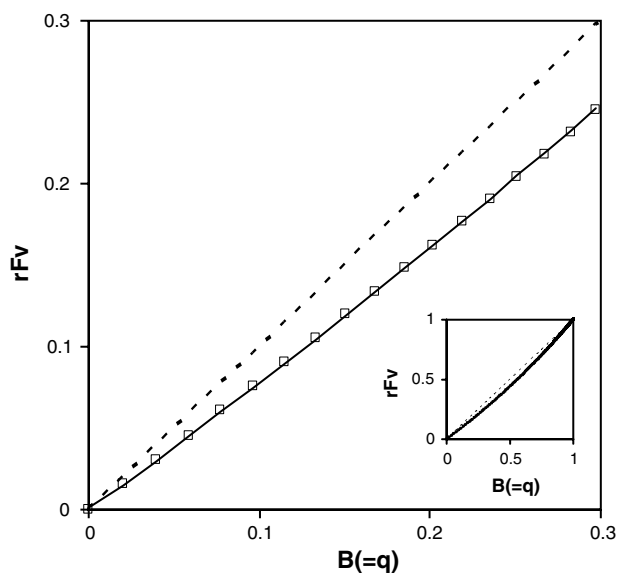
Fig. 3 The relative variable fluorescence yield rFv(t) (Eq. C.3 in Appendix C) plotted against the corresponding normalized area B(t) (Eq. C.4) above rFv(t) (solid line) in the B(t) -range from 0 to 0.3, simulated for MTF excitation at excitation rate k_L far below the rate constant k_{s_1} of donor side quenching release and adopting a double hit trapping mechanism. The symbols are for the same virtual situation adopting a single hit trapping mechanism in which rFv = \frac{q}{1+C_{hyp}(1-q)} (Eq. B.1 in Appendix B) with C_{hyp} = 0.30 for a best fit with the solid line. The insert shows the plots in the full range. In this case the best fit between both curves is for C_{hyp} = 0.28 . Dashed curves are for the linear relation rFv = B with C_{hyp} = 0 . B is the fraction q of RCs with Q_A
