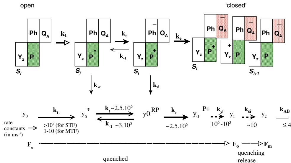
Fig. 1 Upper section. Representation of the reaction pattern and -intermediates associated with light driven transfer of dark-adapted open reaction center (RC) with oxygen evolving complex (OEC) in state S_i (designated with state S_i [ Y_zP Phe Q_A ]) into its first quasi-stationary 'closed' state S_{i+1} [ Y_zP Phe Q_A^- ] in green cells and chloroplasts. The term 'closed' refers to the indicated state with Q_A^- which in terms of the 'classic' 2-state trapping model is considered to be closed with rFv = 1(Fm^{STF}/Fo \sim 5) ; in terms of TSTM state S_{i+1} [ Y_zP Phe Q_A^- ] has been called a semi-closed state with rFv = 0.5(Fm^{STF}/Fo \sim 3) . Arrows (from left to right) mark the sequence light excitation, charge separation, Q_A reduction, Y_z - and OEC-oxidation with rate constants k_L , k_t , k_e , k_{yi} , and k_{si} , respectively, in which i(i=1, \dots, 4) refers to the state S_i of the OEC. Oxidation of Q_A^- by Q_B is indicated with rate constant k_{AB} . The left-directed horizontal arrow marks charge recombination of radical pair P_{680}^+Phe^- with rate constant k_{-1} . Downward pointing arrows mark energy loss of P_{680}^* and of P_{680}^+Phe^- in a form different from photochemical storage with rate constants k_w and k_d , respectively. P_{680} is considered here as the traditional primary electron donor of PSII, ignoring that the accessory
