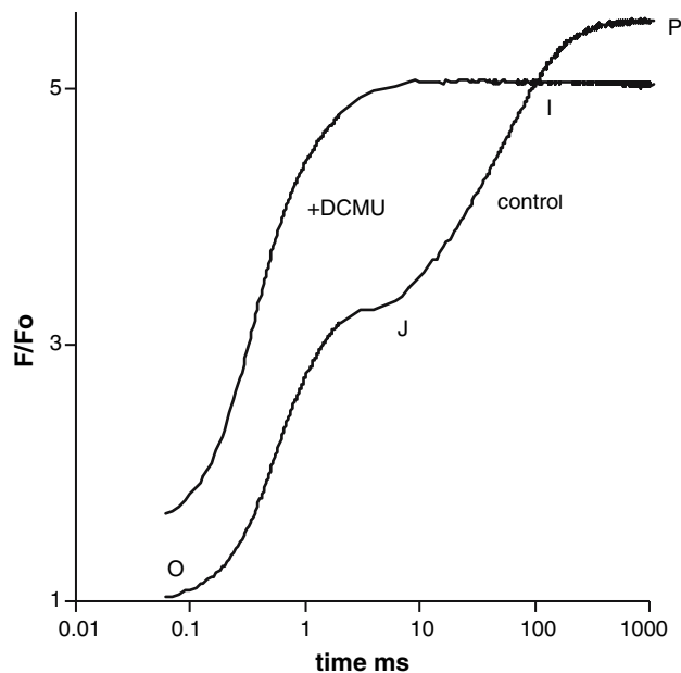
Fig. 4 Direct recordings (average of 3 and plotted on a log time scale) of the fluorescence induction in approximate F/F_0 units of 10–15 min dark-adapted Chenopodium chloroplasts (10 \mu g chl/ml) in a 1 s light pulse in the 0.05 ms to 1 s time range, in the absence (control, OJIP) and presence of 30 \mu M DCMU (+DCMU), respectively. Figure shows (i) the amply documented increase in F(0) (in this case recorded at 0.05 ms) after addition of DCMU relative to F_0 in the absence of the inhibitor with F(0)/F_0 \sim 1.6 , and (ii) decrease in Fm^{MTF}
