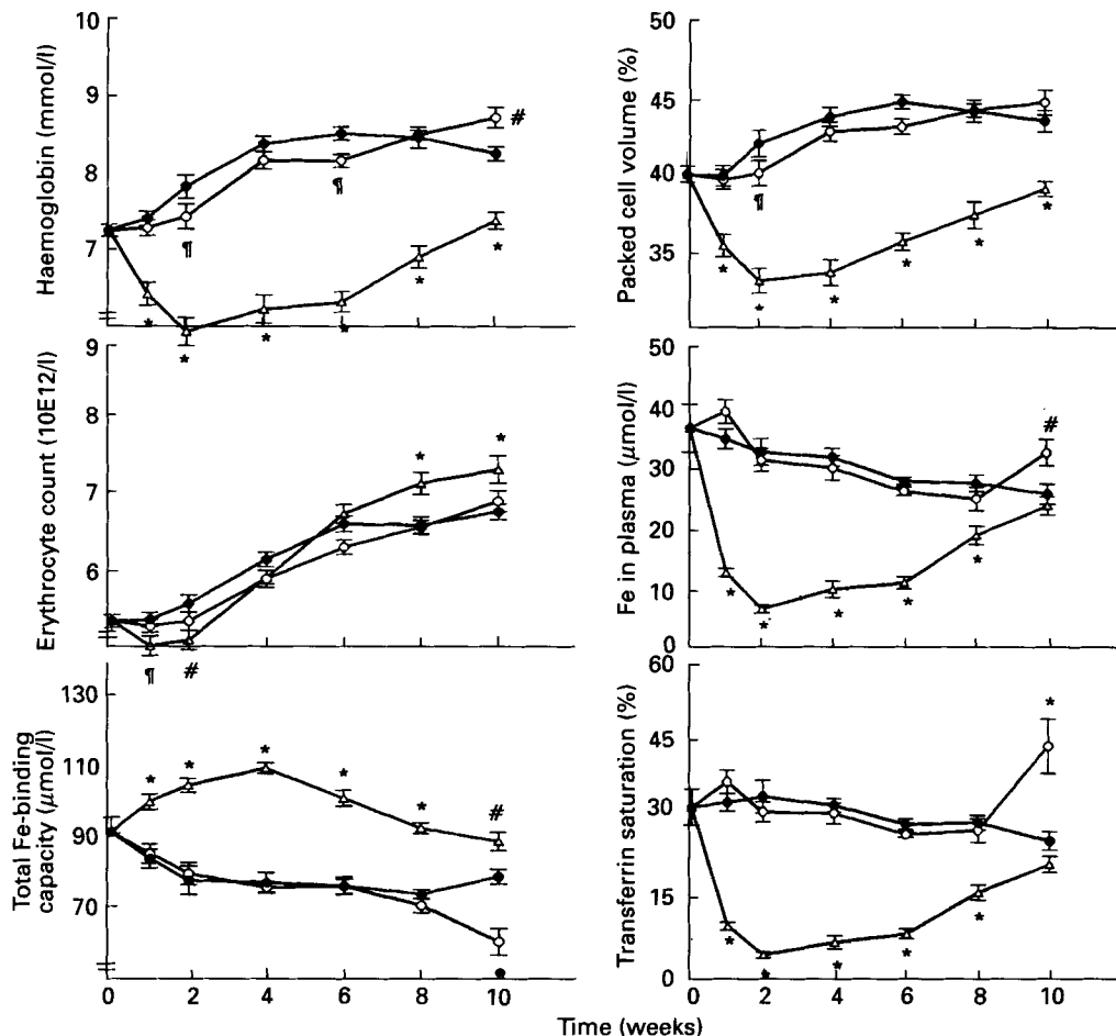
Fig. 3. Time course of haemoglobin concentrations (a), packed cell volume (b), erythrocyte count (c), Fe in plasma (d), total Fe-binding capacity (e) and percentage transferrin saturation (f) in rats given either the control diet (●), vitamin A-deficient diet (○) or Fe-deficient diet (△). Values represent means for twelve rats, with standard errors indicated as error bars. Differences between vitamin A-deficient or Fe-deficient and control groups: ¶ P < 0.05 , # P < 0.01 , * P < 0.001 .
