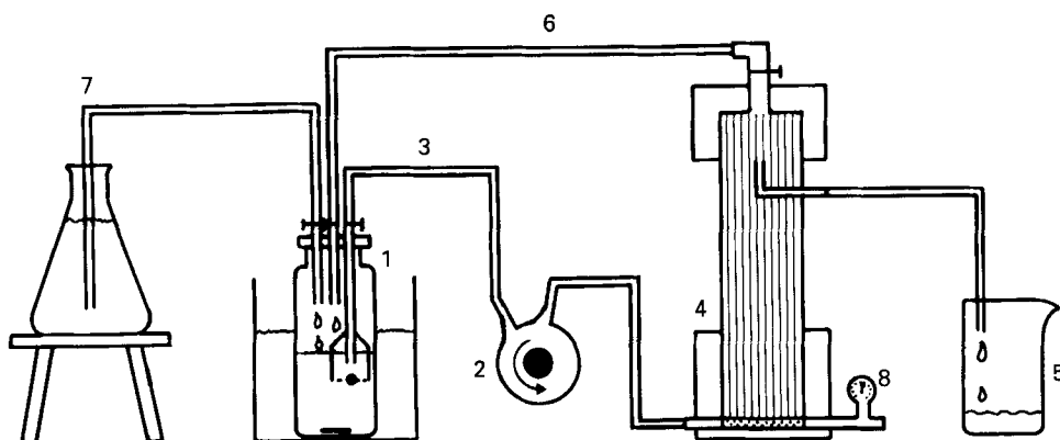
Fig. 1. Schematic representation of hollow-fibre system for continuous dialysis. For details of procedure, see pp. 852–853.
