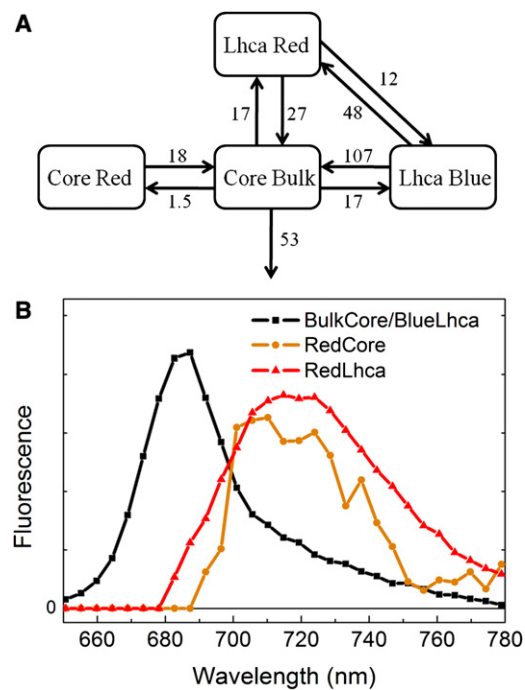
FIGURE 5 Target analysis of PSI-LHCI kinetics. (A) Compartmental model of PSI-LHCI, with EET rates in /ns. (B) Species associated spectra of the compartments.
