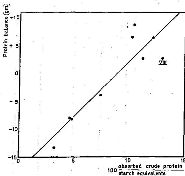
FIG. 1. Correlation between protein balance and absorbed protein per 100 gms. of starch equivalents. (VIII = value obtained in experiment SVIII).
