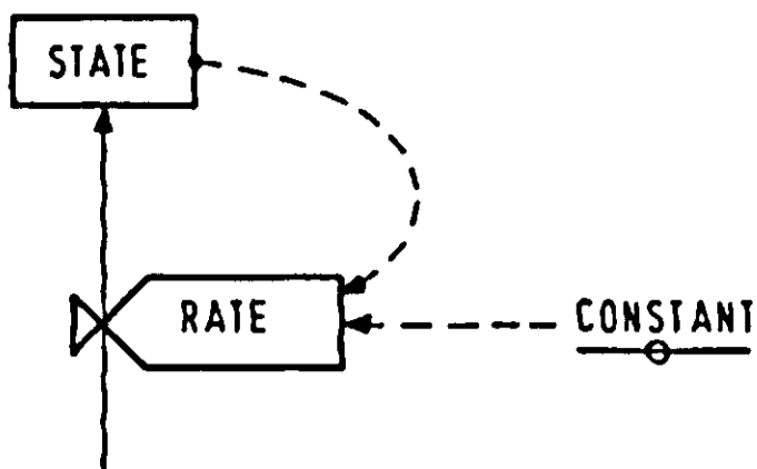
Figure 1. A relational diagram of exponential growth, drawn to the conventions of Forrester (1961).
