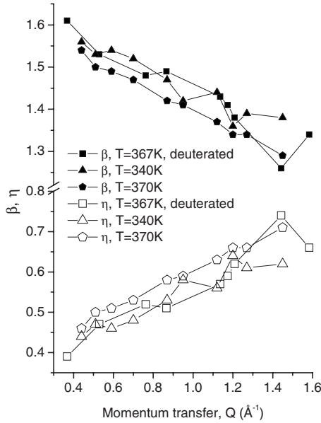
FIG. 6. Dispersion parameter \beta and entropic index, \eta , dependences on momentum transfer, Q , for HAT6 with deuterated tails at T=367 K and HAT6 at temperatures close to the phase transitions T=340 K (crystalline \rightarrow liquid crystalline) and T=370 K (liquid crystalline \rightarrow isotropic).
