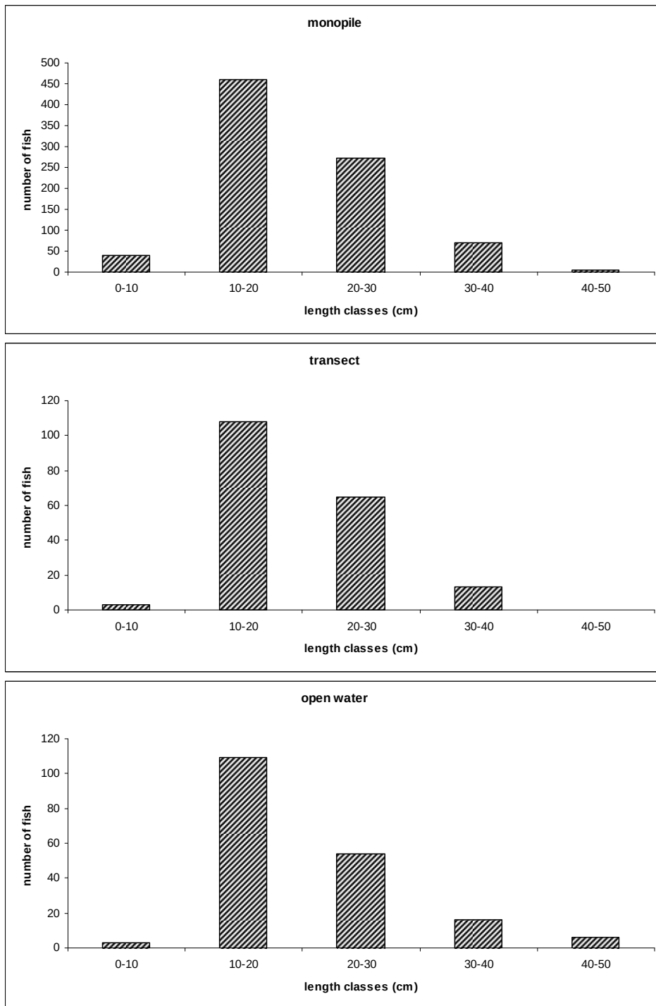
Figure 11. Length distribution of fish around the monopiles as measured from the DIDSON frames.
