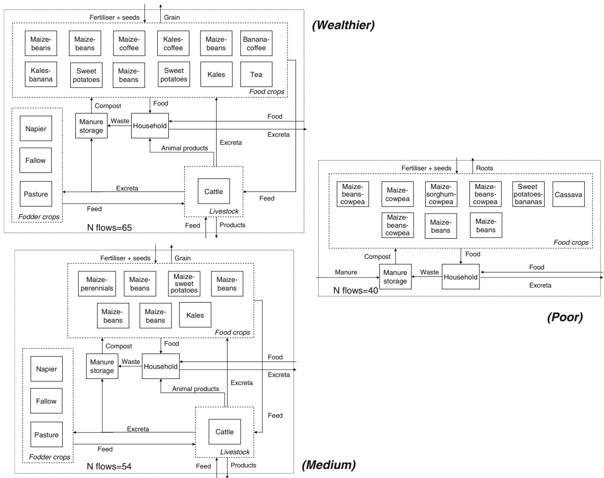
Fig. 4 Schematic representation of the network of N flows for three different farm household types (wealthier, medium and poor) in Mutsulio, Kakamega, western Kenya. The boxes represent compartments conceptualised as farming activities or
