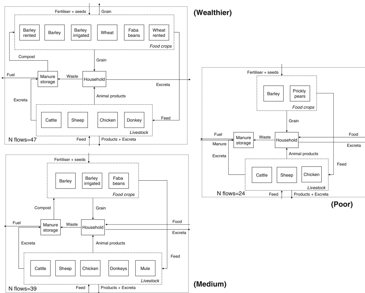
Fig. 2 Schematic representation of the network of N flows for three different farm household types (wealthier, medium and poor) in Teghane, Tigray in the Northern highlands of Ethiopia. The boxes represent compartments conceptualised
