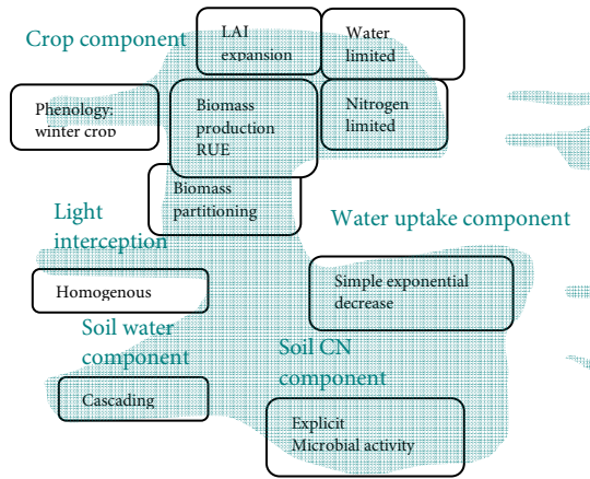
39 Figure 3.1. Representation of APES modularity and flexibility with different levels of granularity: (a) the components, software units used for composition, (b) the modules, conceptualization of a process within a component, (c) the modelling solutions (MS), combination of different modules depending on the objective of the simulation.
