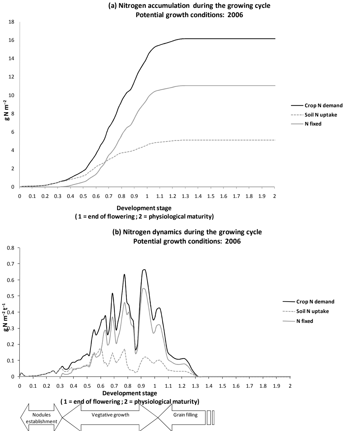
Figure 5.5. Nitrogen dynamics in pea under potential growth conditions*: (a) accumulated crop nitrogen demand, nitrogen uptake from the soil and nitrogen fixation over the growing cycle; (b) daily crop nitrogen demand, nitrogen uptake from the soil and nitrogen fixation over the growing cycle. Integrating Figure 5b gives Figure 5a.
