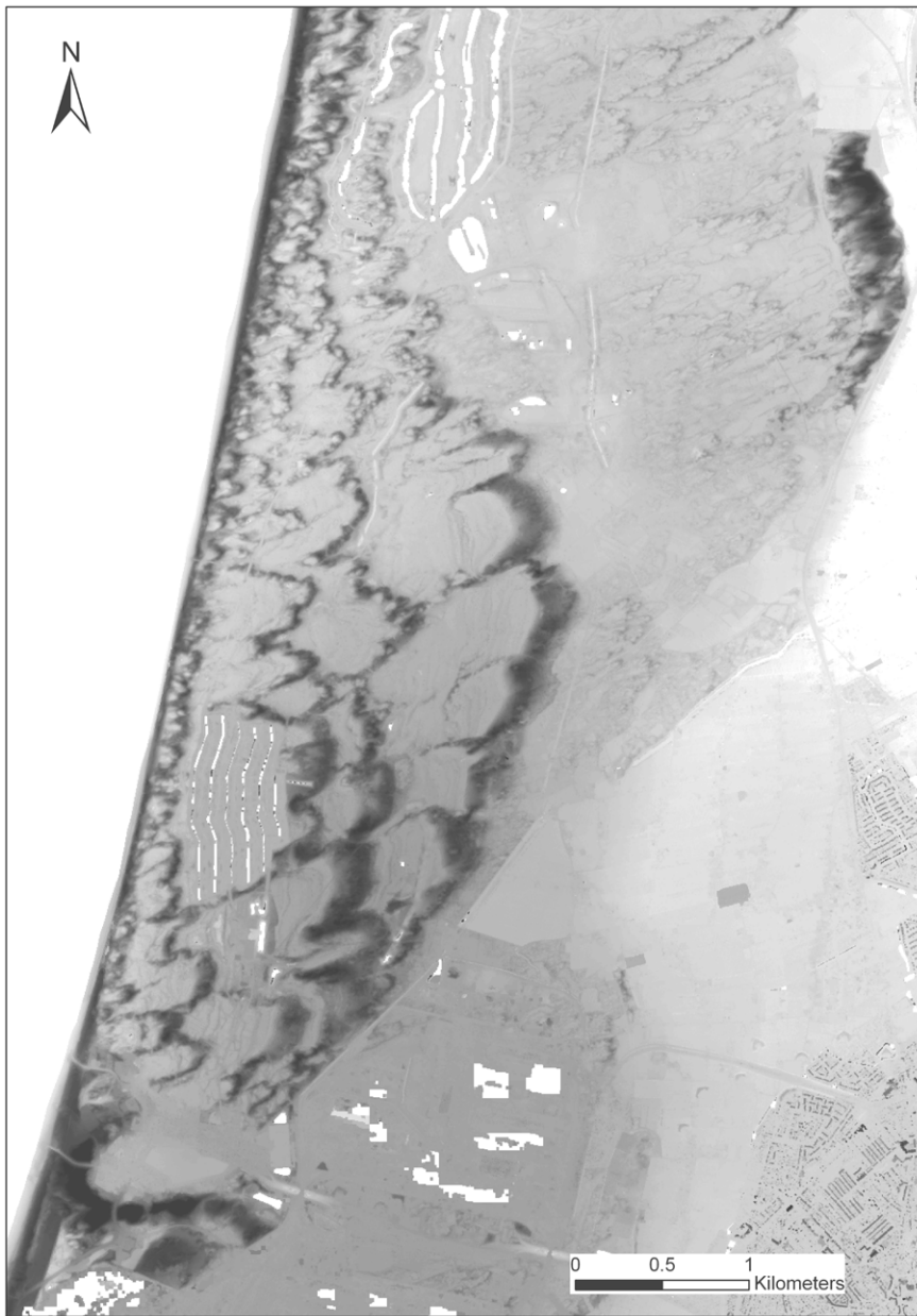
Fig. 6. The comb dunes along the North Sea coast near Castricum . The well-developed ridges on the right side are dated pre-16 th century, allegedly contemporaneous with their counterparts in the inland dunes. Compiled by M. Riksen, data source: AGI-ITC Rijkswaterstaat, 2004.
