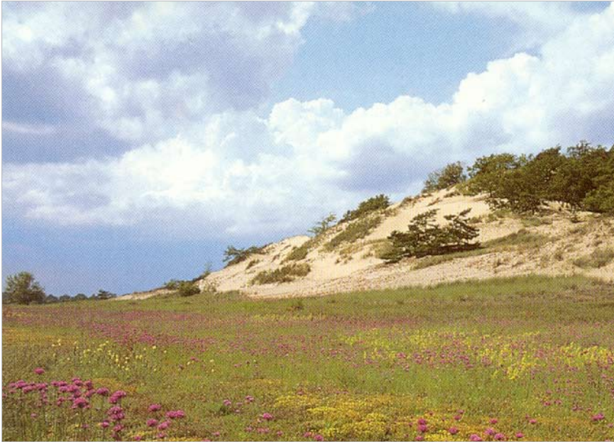
Fig.2. River dune near Dömitz along the Elbe, reactivated by up-hill wind flow acceleration. Photo by P. Jungerius, 2000.
