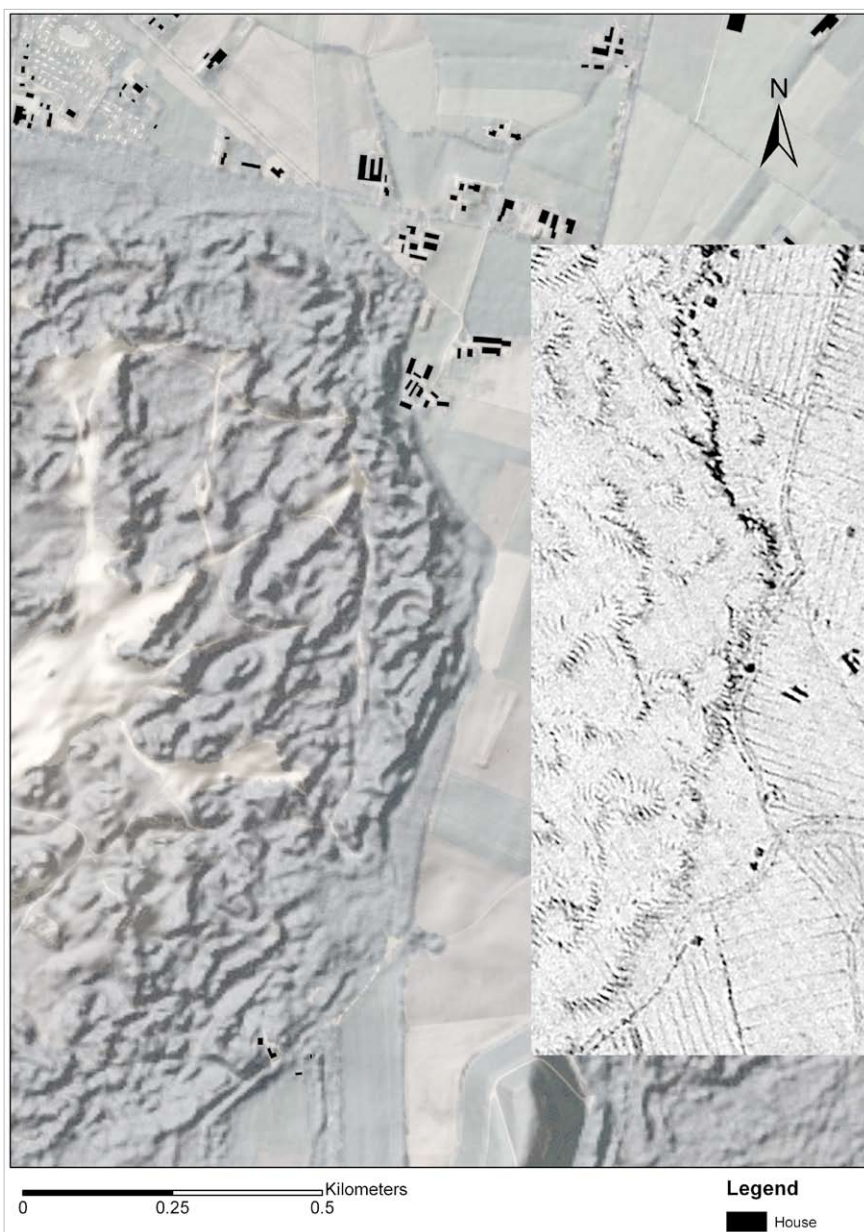
Fig. 8. The NE edge of the Wekeromsezand SW of Wekerom has not shifted between 1802/1810 (insert, De Man 1984) and 2003. Black dots on the insert indicate farms built in the shelter of the terminating dune. Compiled by M. Riksen, aerial photographs: © Eurosense 2003; data source: AGI-ITC Rijkswaterstaat, 2004.
