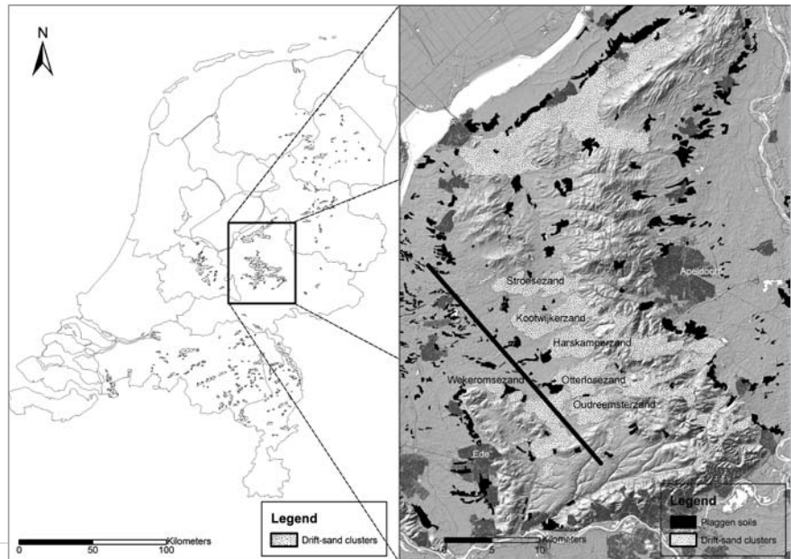
Fig. 5. Left: The drift sand clusters of the Netherlands (light grey). Right: the drift sand clusters (outlined patches) on the flanks of the Veluwe push moraine ridges on both sides of a former glacial valley (arrow). The agricultural fields ("essen") around the settlements with plaggen soils (black) are also indicated. Built-up areas are dark grey. Compiled by M. Riksen, data source: AGI-ITC Rijkswaterstaat, 2004.
