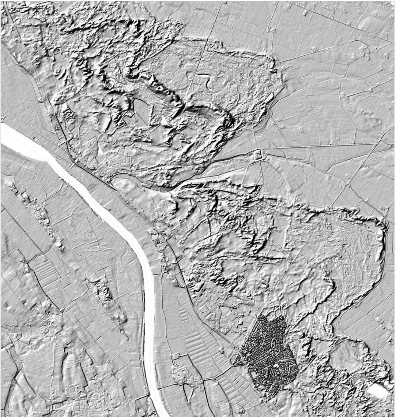
Fig. 7. The superimposed river dunes along the Meuse near Nieuw Bergen . Compiled by M. Riksen, data source: AGI-ITC Rijkswaterstaat, 2004.
