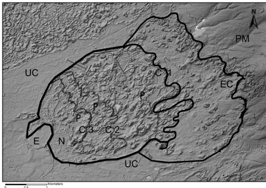
Fig 4. The drift sand cell east of Harskamp , terminating in comb dunes C1. N indicates the zone of nabkhas; P the deflation planes; C2 and C3 mark the comb dune ridges at various stages of windward expansion. Long before the 19 th century the farmers protected their fields E with a wall, to check SW expansion of the drift sand. UC=unaffected old cover sand separating the Harskampse sand from the other clusters; PM=push moraine ridge; EC=terminating comb dunes of preceding cells. Compiled by M. Riksen, data source: AGI-ITC Rijkswaterstaat, 2004.
