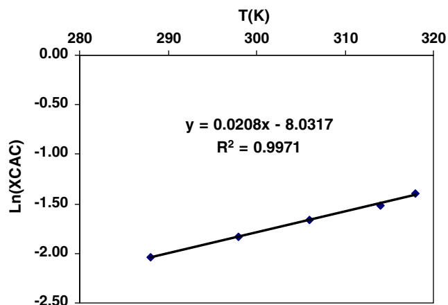
Fig. 5 \ln(x_{1, CAC}) as a function of temperature for calculations of \Delta H^0 using Eq. 3
