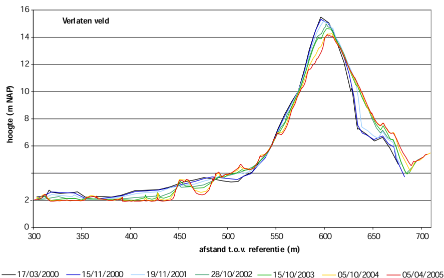
Figure 8 Mobility and change in profile of the parabolic dune.
