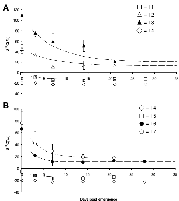
Figure 1 \delta^{13}\text{C} of whole mosquitoes ( \pm standard deviation) against time after emergence (days) for treatments T1-T4 (A) and T4-T7 (B). The dashed lines represent the modeled data.
