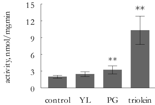
Figure 1. Transketolase activity in livers of 19 day old embryos. Values shown are means \pm standard error over 13, 8, 6 and 4 individuals for controls, yolk lipids (YL), propylene glycol (PG) and triolein, respectively. **, significantly different from control ( p < 0.01 ).
