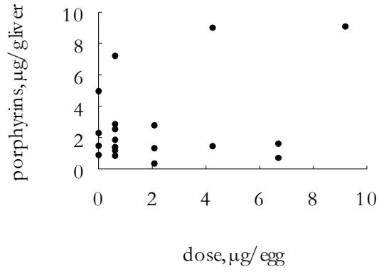
Figure 2a. Hepatic porphyrin concentration in 19 day old embryos exposed to increasing concentrations of hexachlorobenzene.
